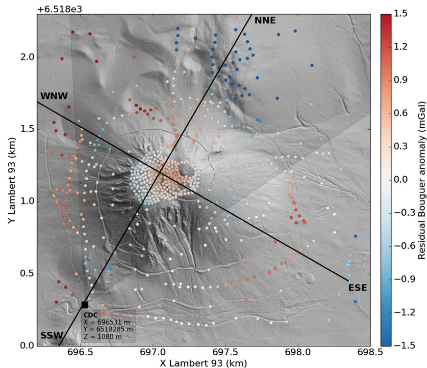
FIGURE 2 | Residual Bouguer anomaly data of the Puy de Dôme volcano using correction densities of 2,670 \text{ kg/m}^3 (far-field), 2,420 \text{ kg/m}^3 (mid-field) and 1,890 \text{ kg/m}^3 (near-field). The gravimetric measurements are from Portal et al. (2016). The extent of this map is indicated by a blue square in Figure 1 . The location of the muon detector installed at the Col de Ceyssat (CDC) is indicated (black square) as well as the angle of view of the detector (gray shaded area). The two black lines locate the slices of the inversion results shown in Figures 6, 7 .
