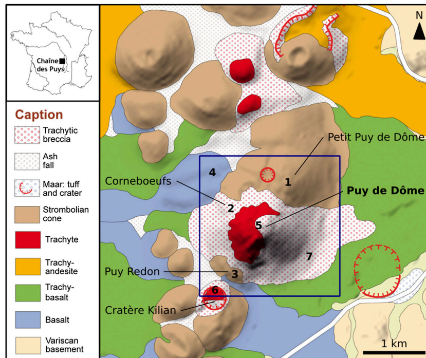
FIGURE 1 | Simplified geological map of the Puy de Dôme and neighboring cones, adapted from Boivin et al. (2017). Top left: Location of the Chaîne des Puys in France. Blue square: Study area of the present paper (Figures 2, 7).
