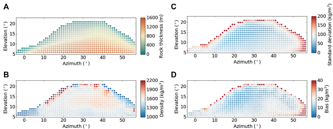
FIGURE 3 | Preliminary muographic data of the Puy de Dôme volcano as observed from the Col de Ceyssat with the TOMUVOL detector and associated errors (Cârloganu and the TOMUVOL collaboration, 2018; Niess et al., 2018a). The location of the muon detector is indicated in Figure 2 . (A) Thickness of rock along the muon trajectories. (B) Averaged densities estimated from the muon count. (C) Statistical error (i.e., standard deviation). (D) Systematic error (i.e., bias).
