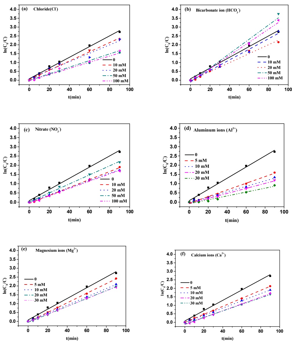
289 Fig. 5. Effect of inorganic anions and cations on MB degradation under simulated solar light irradiation 290 (a-e). Experimental condition : [\text{MB}] = 20 \text{ mg}\cdot\text{L}^{-1} , [\text{5 wt\% Fe-C}_3\text{N}_4] = 0.5 \text{ g}\cdot\text{L}^{-1} , no pH adjustment and 291
