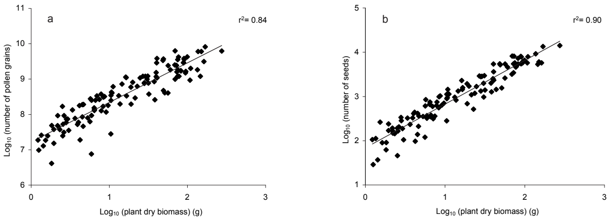
Figure 2. Relationships between \text{Log}_{10} (plant dry biomass) and \text{Log}_{10} (number of pollen grains) (a) or \text{Log}_{10} (number of seeds) (b) of 121 common ragweed plants from five French natural populations. Linear regression lines (—) and coefficient ( r^2 ) are shown on the diagrams.
