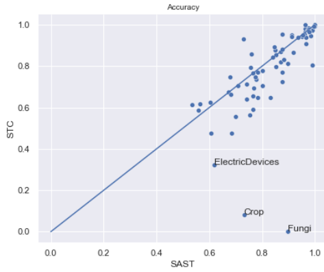
(a) SAST (43 wins) vs STC (27 wins), 2 draws
