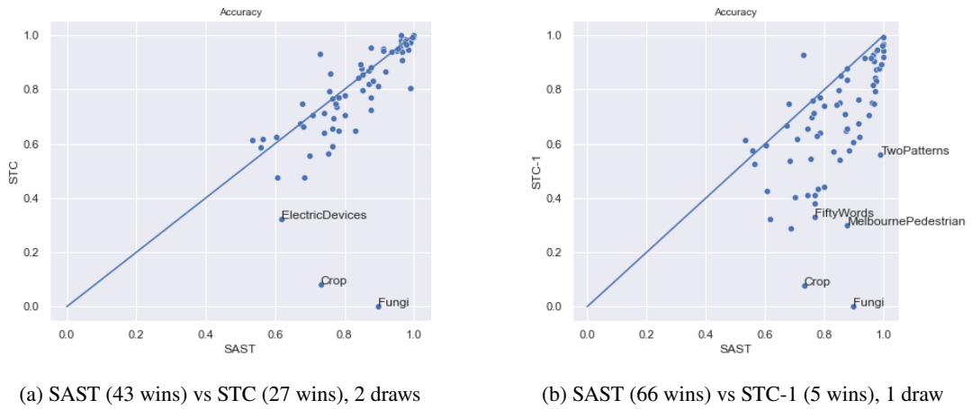
Figure 13: Pairwise comparison of SAST, STC and STC-1
