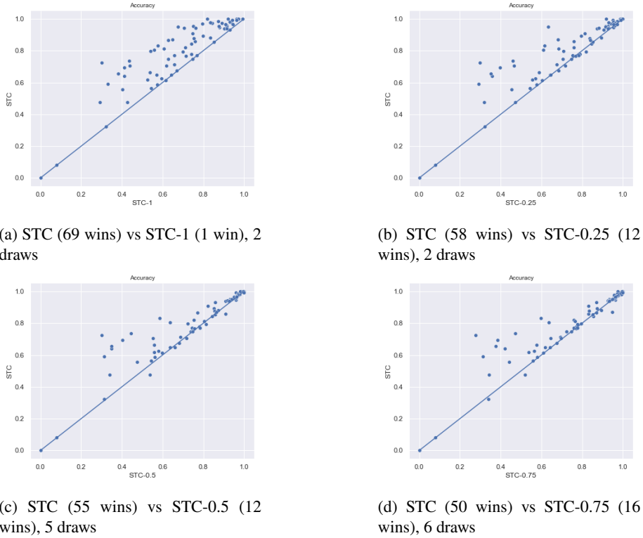
Figure 8: Comparison of STC-k to STC in terms of accuracy
