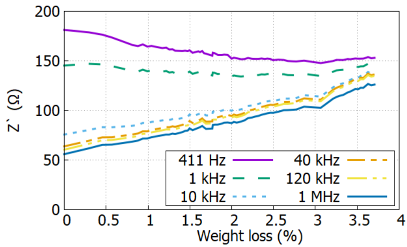
Fig. 9: Real impedance of low-fiber mortar as a function of (a) Time, (b) Shrinkage and (c) Weight loss
