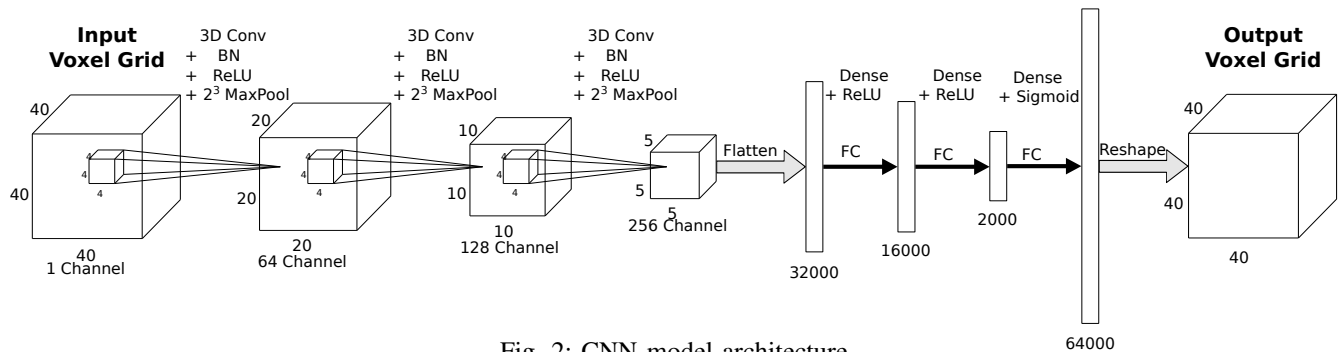
Fig. 2: CNN model architecture
