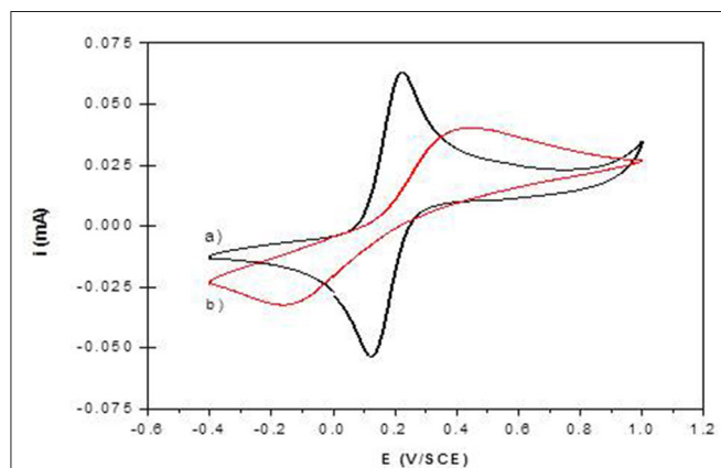
FIGURE 7 | Cyclic voltammograms of 1 mM \text{K}_4\text{Fe(CN)}_6 in 0.1 M Tris buffer (pH 7) recorded at (a) NiAl@Alg-Ca/ITO and (b) NiAl- \text{CO}_3 /ITO ( v = 50 \text{ mVs}^{-1} ).
