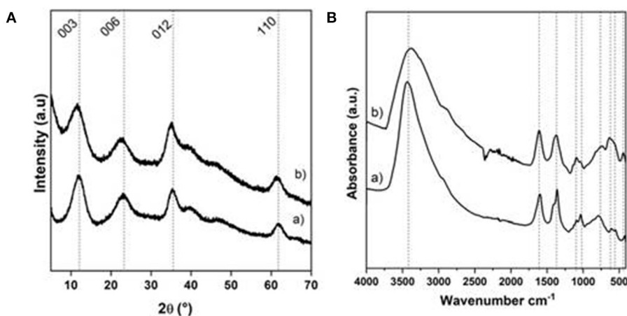
FIGURE 3 | (A) PXRD patterns and (B) FTIR spectra of (a) NiAl@Alg-Ca beads and (b) NiAl@Alg beads dried upon CO 2 supercritical conditions.
