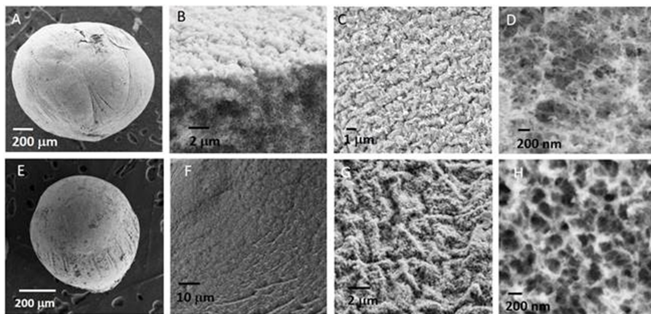
FIGURE 2 | SEM images of (A–D) NiAl@Alg-Ca beads and (E–H) NiAl@Alg beads dried upon CO 2 supercritical conditions.
