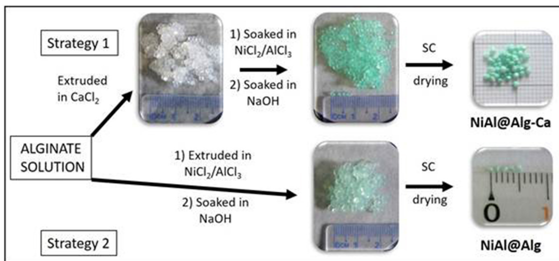
FIGURE 1 | Scheme of preparation of NiAl nanoparticles confined in Alg beads using either Ca-Alg as a template for confined LDH coprecipitation (Strategy 1) or alginate cross-link by \text{NiCl}_2 and \text{AlCl}_3 metal salt solution (Strategy 2). For both strategies, the LDH coprecipitation was induced by soaking in a NaOH (1 M) solution and bionanocomposite beads were dried in \text{CO}_2 supercritical conditions.
