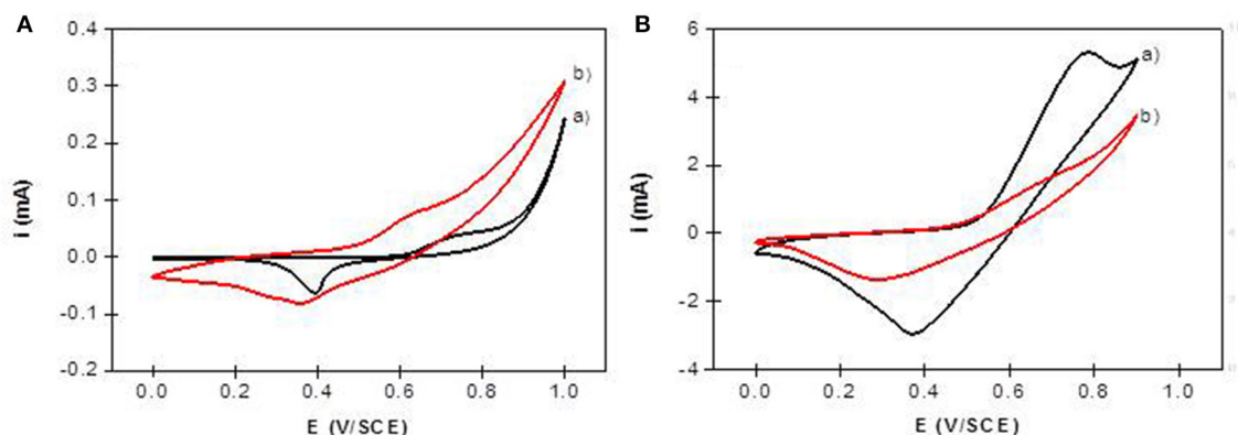
FIGURE 9 | Cyclic voltammograms recorded in 0.1 M NaOH ( \nu = 50 \text{ mVs}^{-1} ) using (A) NiAl- \text{CO}_3 /ITO (curve a) and NiAl-Alg/ITO (curve b) modified electrodes prepared by solvent casting; (B) NiAl@alginate composite electrodes prepared by impregnation (a) NiAl@Alg-Ca/ITO and (b) NiAl@Alg/ITO.
