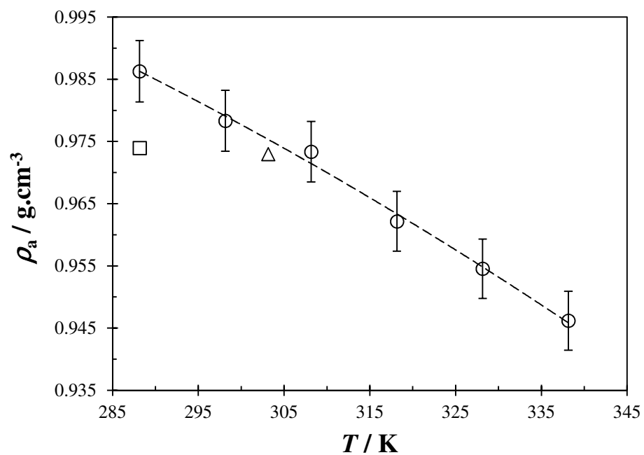
Figure 4. Comparison of densities of pure DMP-30 as function of temperature from this work with values available in the literature: \circ , this work; \square , Bruson and MacMullen [24]; \triangle , Bondi and Parry [25]. Dashed lines, connecting line.
