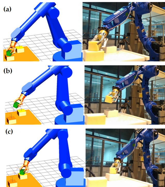
Figure 11. Pick-and-place of the cube by the Adept robot and the Barrett hand: (a) grasping, (b) lifting, and (c) leaving.
