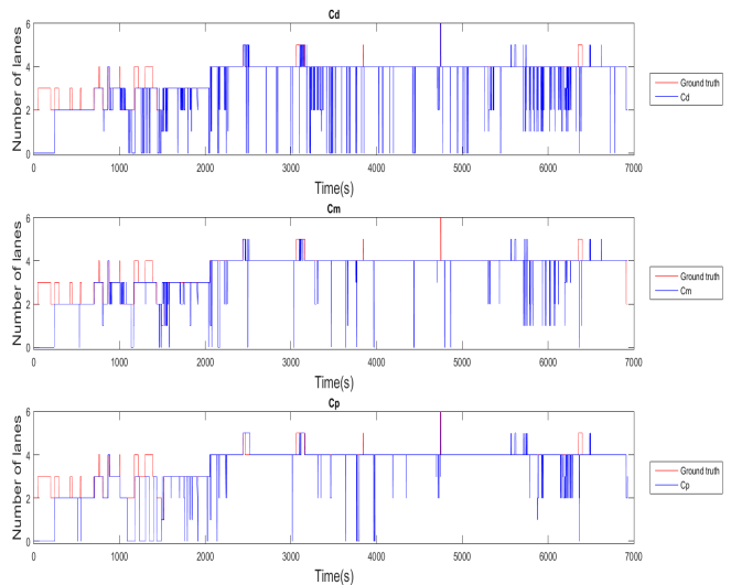
Fig. 8: Lanes estimation compared to ground truth for every criterion used in the map matching.
