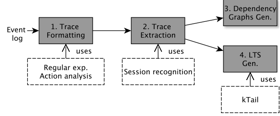
Figure 2: Model learning with the CkTail approach
