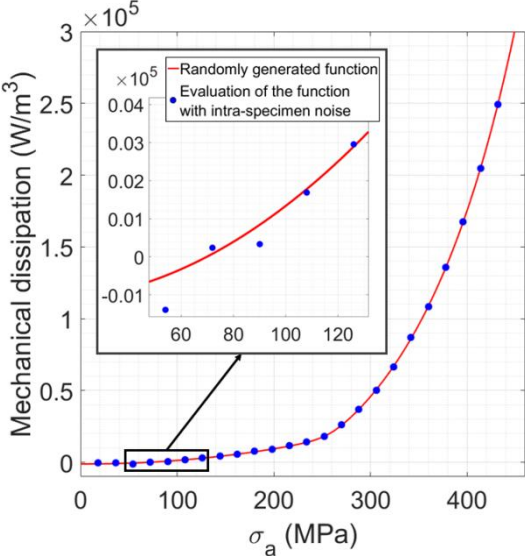
Fig. 12. Example of data set generation for one numerical specimen: mechanical dissipation as a function of stress amplitude \sigma_a .
