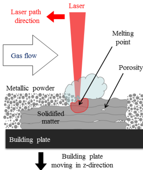
Fig. 1. Principle of the L-PBF manufacturing.
