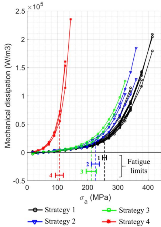
Fig. 14. Application to compare four manufacturing strategies: mechanical dissipation as a function of stress amplitude \sigma_a .
