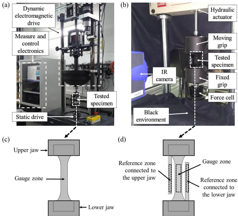
Fig. 3. (a) Experimental setup for conventional fatigue tests; (b) experimental setup for fatigue tests instrumented with IR camera; (c) schematic view of the specimen geometry in the jaws of the testing machine for conventional fatigue tests; (d) same for fatigue tests instrumented with IR camera.
