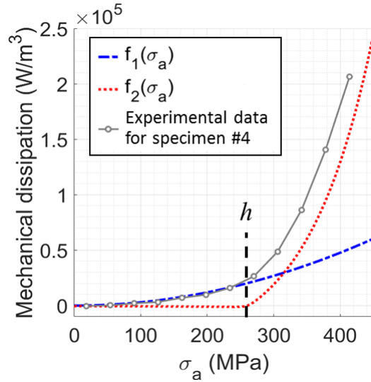
Fig. 10. Illustration of the model fitted to the Specimen #4 data set: functions f_1 and f_2 describe the mechanical dissipation behavior as a function of the stress amplitude \sigma_a .
