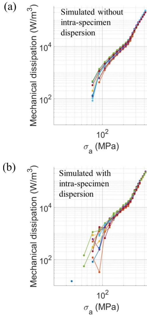
Fig. 13. Group of 14 simulated data sets (a) without and (b) with intra-specimen dispersion: mechanical dissipation as a function of stress amplitude \sigma_a . Note that negative mechanical dissipation values at low loading levels (due to intra-specimen noise) are not displayed in logarithmic scale.
