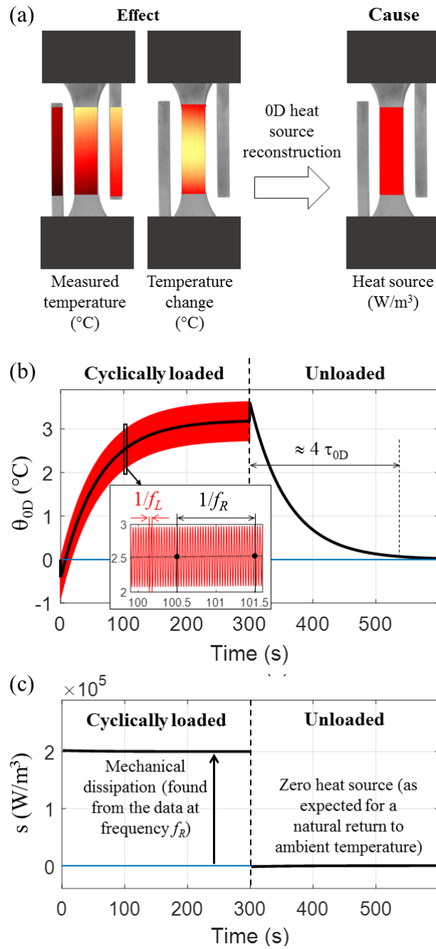
Fig. 7. Data processing approach for the fatigue tests instrumented by IR camera: (a) illustration of the 0D approach; (b) time variation of the spatially-averaged temperature change under cyclic mechanical loading for 300 s, followed by a natural return to ambient temperature; (c) corresponding time variation of the heat source calculated from the data averaged in time over an integer number of mechanical cycles. The input thermal data in this figure was provided by a numerical model.
