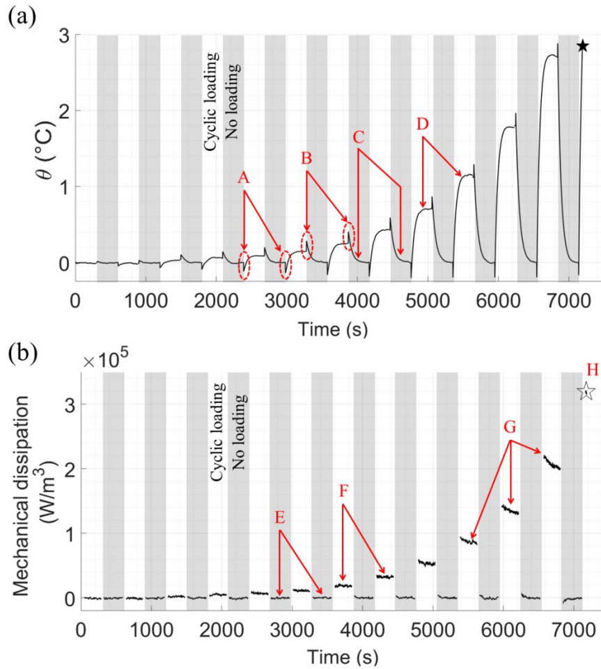
Fig. 8. Typical result of fatigue test instrumented with IR camera, for specimen #9: (a) averaged temperature change as a function of time; (b) mechanical dissipation as a function of time.
