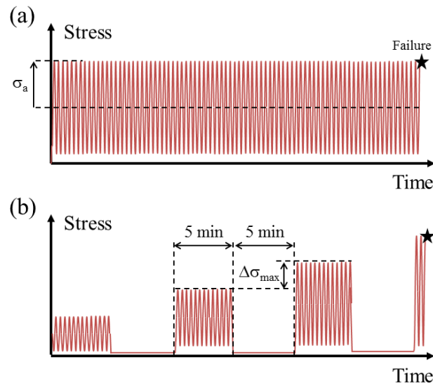
Fig. 4. Schematic view of the mechanical loading: (a) for conventional fatigue tests; (b) for fatigue tests instrumented with IR camera.
