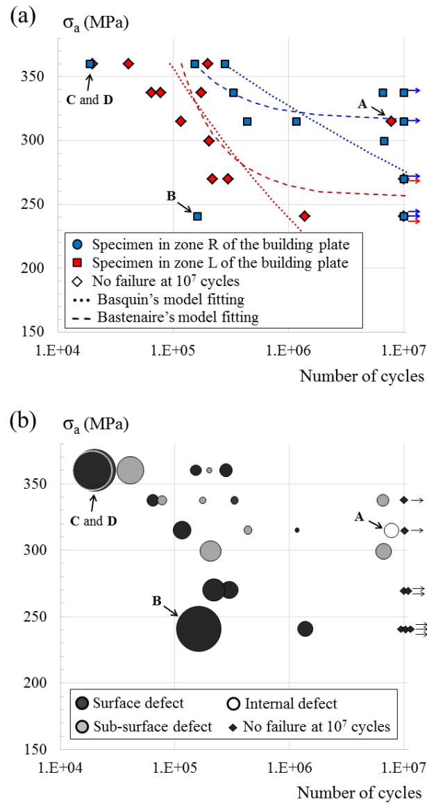
Fig. 5. S-N data plots obtained from the conventional fatigue tests: (a) comparison between specimens placed in the L and R zones of the building plate during manufacturing; (b) comparison between the types of defects observed in the failure zone of the broken specimens. The diameter of the circles is proportional to the area of the defect.
