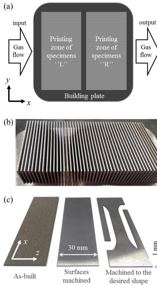
Fig. 2. Specimen manufacturing: (a) schematic view of the two printing zones on the building plate; (b) photograph of as-built plates on the building plate; (c) photograph of specimens at different manufacturing stages.
