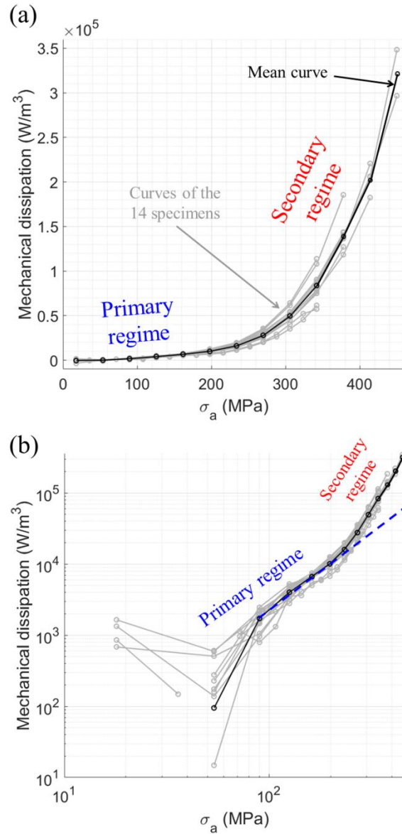
Fig. 9. (a) Mechanical dissipation vs. stress amplitude for the 14 tested specimens; (b) same in log-log plot.
