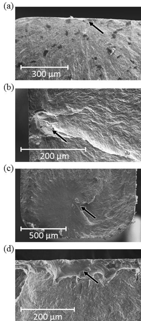
Fig. 6. SEM micrographs of four representative fracture initiation sites after conventional fatigue tests: (a) small surface defect; (b) medium sub-surface defect; (c) small internal defect; (d) large surface defect.
