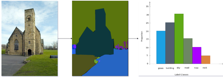
Fig. 4. Semantic histogram
