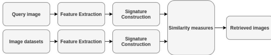
Fig. 1. Cbir system
