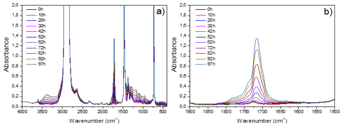
Fig. 6 - a) Infrared spectra of a 80 μm-thick PEr film during thermal oxidation at 110°C; b) in the region between 1900 and 1500 cm -1 .
