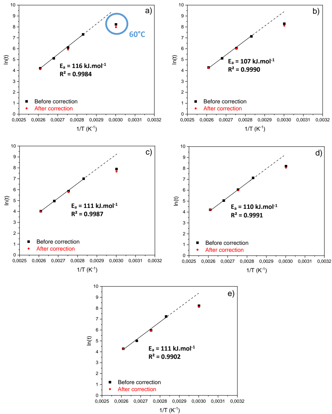
Fig. 12. Arrhenius plot of the ageing time t corresponding to \Delta\text{Absorbance} = 0.5 (before and after correction by the amorphous phase fraction) for a) PEr b) 7030r c) 5050r d) 3070r e) PEcBr.
