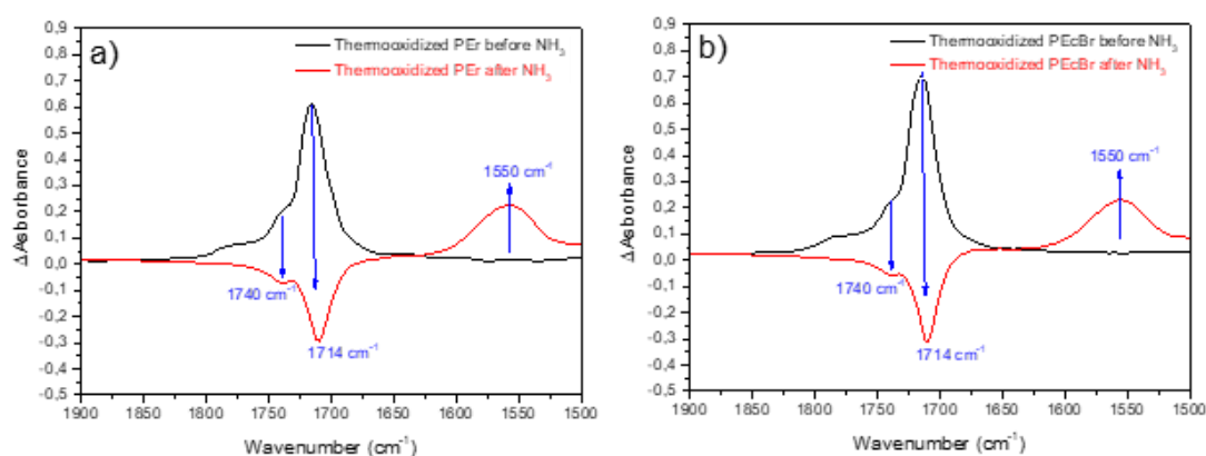
Fig. 7 – Subtracted FTIR spectra ( A_t - A_0 ) of thermo-oxidized PEr (a) and PEcBr (b) films before and after treatment with \text{NH}_3 .
