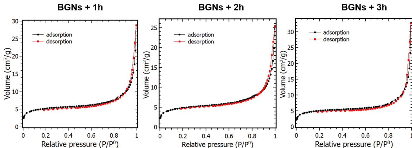
Figure 2. Adsorption-desorption isotherms of BGNs+1h, BGNs+2h and BGNs+3h.
