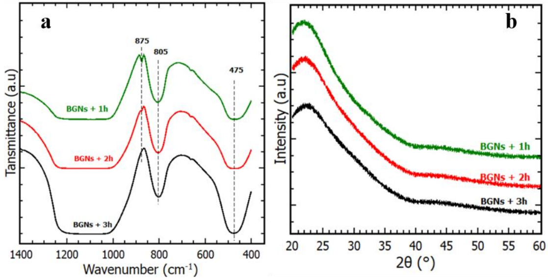
Figure 4. a) IR spectra and b) XRD patterns of BGNs.
