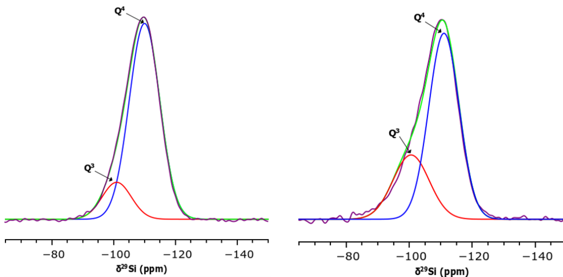
Figure 3. Experimental ^{29}\text{Si} RMN spectra of 100Si (left) and BGNs+2h (right) fitted with Gaussian functions corresponding to \text{Q}^4 units (blue) and \text{Q}^3 units (red). The green curves correspond to the sum of these 2 Gaussians.
