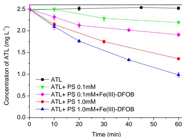
Fig. 2 Degradation of ATL in Fe(III)-DFOB/PS system under simulated sunlight irradiation
