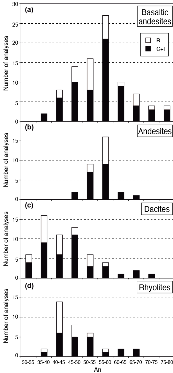
Figure 7. Histograms of An contents for plagioclases derived from (a) basaltic andesites, (b) andesites, (c) dacites, and (d) rhyolites. Rims (R) are differentiated from core and interior (C+I) compositions. Note the large An variations, namely for plagioclase from the BA group, and the fact that most compositions in the BA (and andesites) display An 55-65 , whereas the plagioclases in the dacites and rhyolites are generally between An 35-50 .
