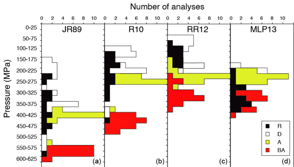
Figure 11. Histograms of amphibole crystallization pressure estimates for Ubina samples (BA: basic andesites; A: andesites; D: dacites; R: rhyolites). Different models have been tested (JR89: Johnson and Rutherford, 1989; R10: Ridolfi et al., 2010; RR12: Ridolfi and Renzulli, 2012; MLP: Médard and Le Pennec, 2013).
