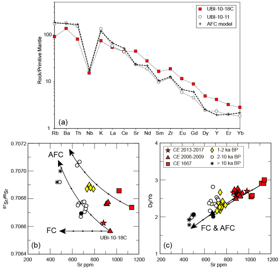
Figure 13. Results of the geochemical modelling. (a) Multielement diagram normalized to Primitive Mantle (Sun and McDonough, 1989) for the mafic (UBI-10-18C) and silica-rich (UBI-10-11) end-members, as well as an AFC model. (b) Sr vs. ^{87}\text{Sr}/^{86}\text{Sr} diagrams showing the Ubina samples as well as the AFC and FC models from two mafic end-members (UBI-10-18C and UBI-99-10). (c) Sr vs. Dy/Yb diagram for Ubina samples and the two AFC models. The fractionating phases for both models (FC and AFC) are 46% Pl + 44% Amph + 3% Cpx + 6% Mag + 1% Apt, and the assimilation/fractional crystallization rate ( r ) = 0.04. Partition coefficients were compiled by Rivera et al. (2017) and correspond to intermediate to acid liquids. Note that in (a) and (c) AFC and FC models display almost the same values due to the fact that trace elements are slightly modified by the very low degrees of crustal assimilation, whereas in (b) we clearly show that assimilation is needed to explain the Sr isotopic variation. Symbols are the same as in Fig. 3.
