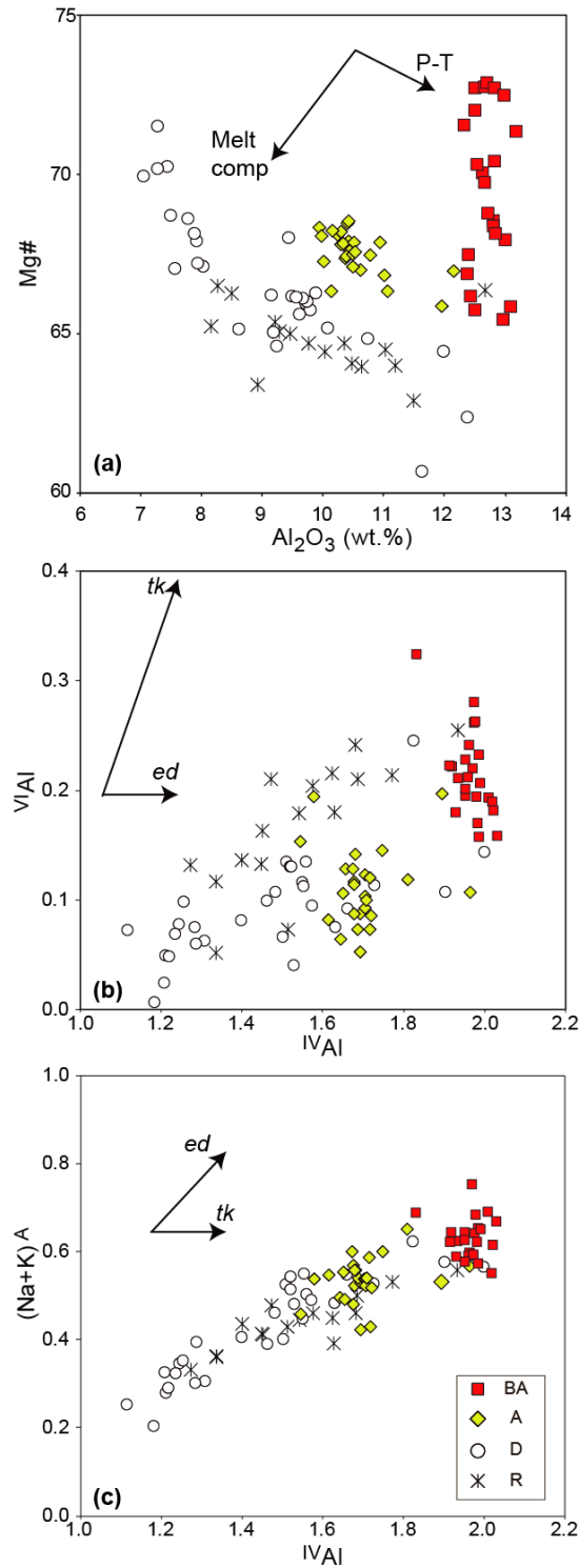
Figure 8. (a) Diagram showing the \text{Al}_2\text{O}_3 and Mg# variations for Ubina amphiboles. The vectors represent in a schematic way the effect of an increase in P-T as well as a variation of mafic to felsic magma chemistry (modified from Kiss et al., 2014). (b) \text{IVAl} vs. \text{VIAl} , and (c) \text{IVAl} vs. (\text{Na}+\text{K})^{\text{A}} showing the effect of edenite ( ed ) and tschermakite ( tk ) substitutions (after Poli and Schmidt, 1992).
