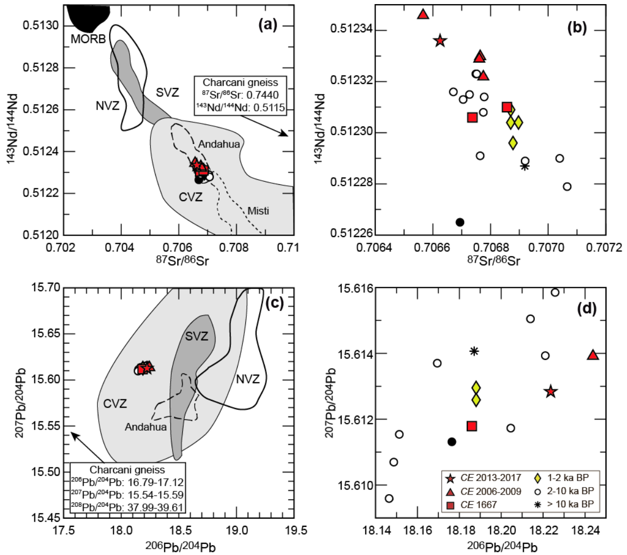
Figure 5. (a) ^{87}\text{Sr}/^{86}\text{Sr} vs. ^{143}\text{Nd}/^{144}\text{Nd} diagram for Ubinas rocks, compared with published isotopic data for the Mid-Ocean Ridge Basalts (MORB, White et al., 1993 and reference therein) and the Andean Northern, Central and Southern Volcanic Zones (NVZ, CVZ and SVZ respectively; Davidson et al., 1991; Ancellin et al., 2017). (b) Detailed ^{87}\text{Sr}/^{86}\text{Sr} vs. ^{143}\text{Nd}/^{144}\text{Nd} diagram for Ubinas samples. (c) ^{206}\text{Pb}/^{204}\text{Pb} vs. ^{207}\text{Pb}/^{204}\text{Pb} diagram for Ubinas samples. Note the extreme homogeneity of Ubinas volcano compared to the very large field displayed for the CVZ. (d) Detailed ^{206}\text{Pb}/^{204}\text{Pb} vs. ^{207}\text{Pb}/^{204}\text{Pb} diagram for Ubinas samples. The absence of linear correlation suggests that a process more complicated than a simple binary mixing process controls Pb isotopes variations. Data from the Andahua monogenetic cones (Delacour et al., 2007) and El Misti volcano (Rivera et al., 2017) are also included. The isotopic signature of the Precambrian Charcani gneiss comes from Boily et al. (1990), Mamani et al. (2010) and Rivera et al. (2017). Symbols are the same as in Fig. 3. Analytical error bars are within the symbol size.
