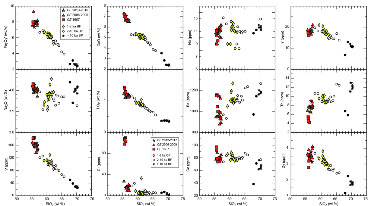
Supplementary material 5. Binary diagrams of the Ubina magmatic series, showing major (Fe 2 O 3 *, CaO, Na 2 O, TiO 2 ) and trace elements (V, Cr, Nb, Y, Ba, Th, Ce, Dy) plotted against silica as a differentiation index.
