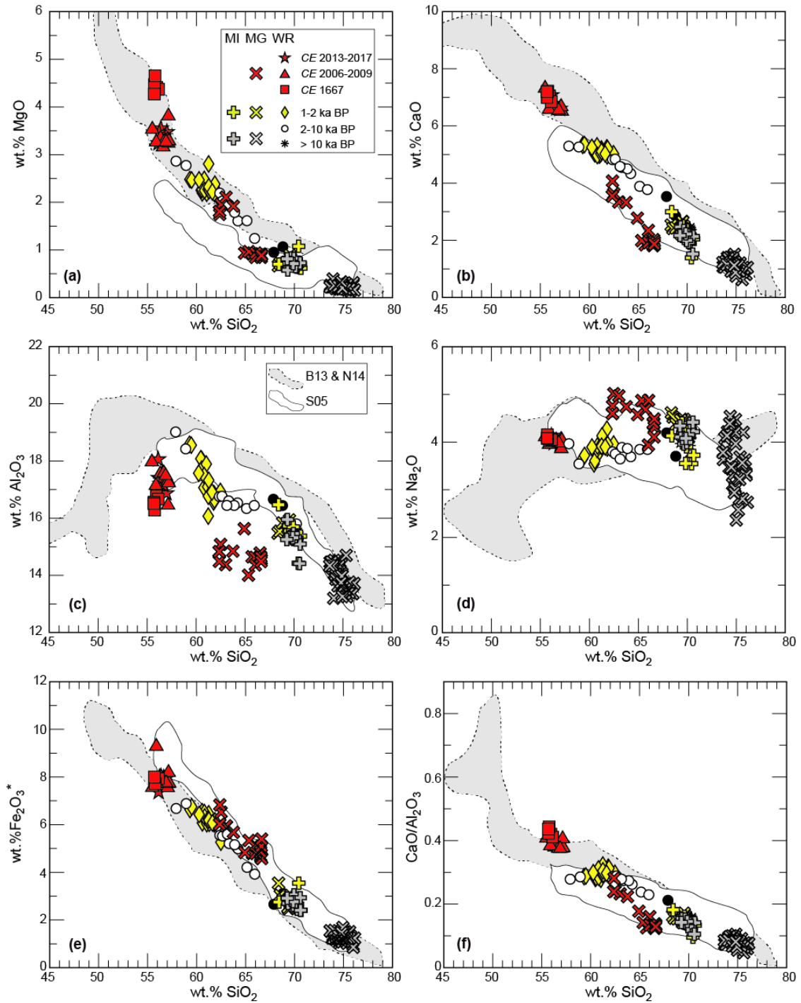
Figure 10. MgO (a), CaO (b), Al 2 O 3 (c), Na 2 O (d), Fe 2 O 3 * (e), CaO/Al 2 O 3 (f) as a function of silica for whole-rocks (WR), matrix glasses (MG) and melt inclusions (MI) of Ubina samples. The fields of experimentally determined liquid-line-of-descent compositions are shown for comparison (S05: Sisson et al., 2005; B13: Blatter et al., 2013; N14: Nandedkar et al., 2014).
