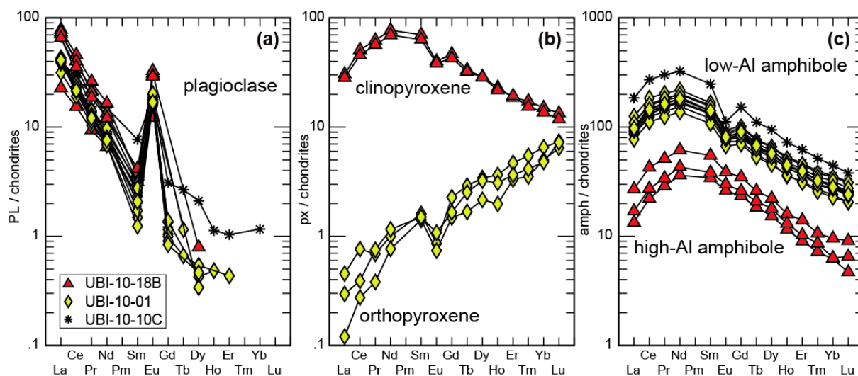
Figure 9. Rare earth element (REE) diagram for selected (a) plagioclase, (b) ortho and clinopyroxene, and (c) amphibole phenocrysts from Ubinas samples. Note that two populations exist for amphibole. Data normalized to chondrite values (Sun and McDonough, 1989). Data correspond to a basaltic andesite (UBI-10-18B), an andesite (UBI-10-01) and a rhyolite (UBI-10-10C).
