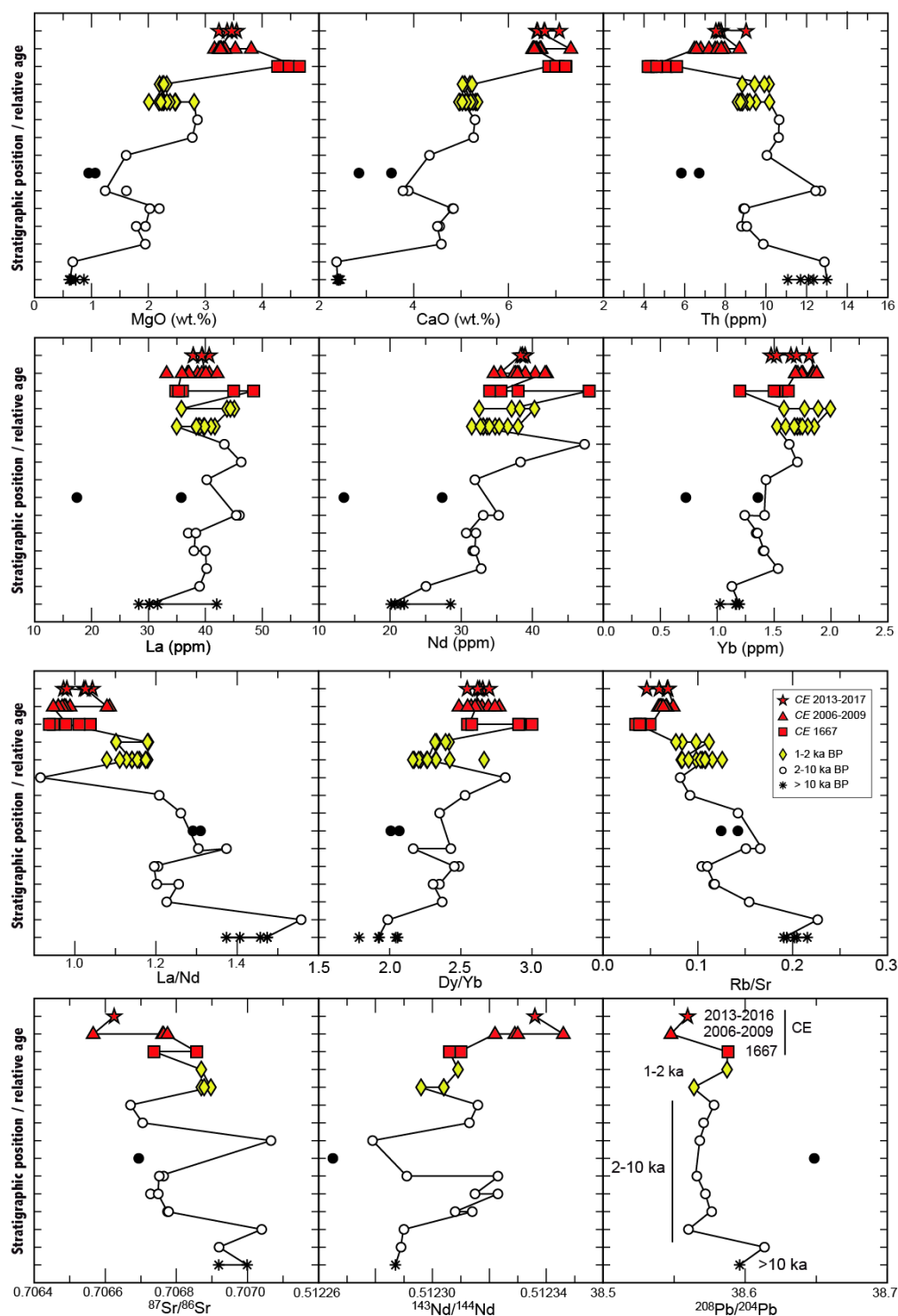
Supplementary material 6. Temporal variation of the Ubina magmatic series, showing some key major (MgO and CaO), trace elements concentrations (Th, La, Nd, Yb) and ratios (La/Nd, Dy/Yb, Rb/Sr), as well as some isotopic ratios ( ^{87}\text{Sr}/^{86}\text{Sr} , ^{143}\text{Nd}/^{144}\text{Nd} , ^{208}\text{Pb}/^{204}\text{Pb} ).
