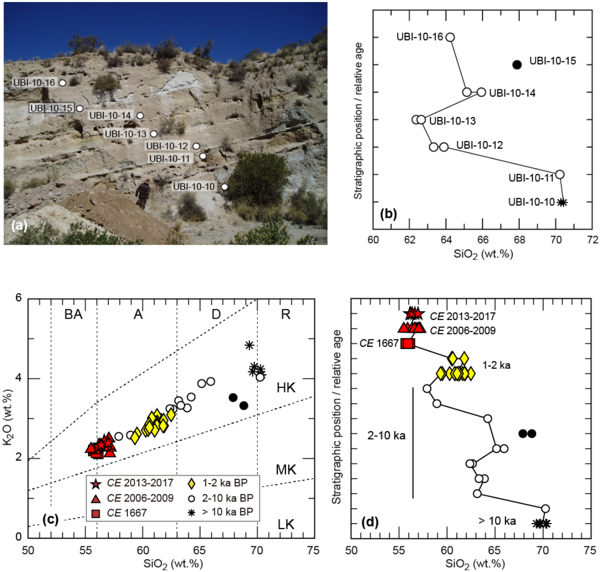
Figure 3. (a) Sample locations on the Sacuhaya cross-section. (b) Silica content of samples from the Sacuhaya section. (c) K 2 O vs. SiO 2 diagram from the post-glacial, historical, and recent samples of Ubina volcano. The fields in this diagram are taken from Peccerillo and Taylor (1976). BA, basic andesite; A, andesite; D, dacite; R, rhyolite; LK, low potassium; MK, medium potassium; HK, high potassium. (d) Silica contents vs. stratigraphic position for the post-glacial to recent samples. Black dots correspond to samples from a distal tephra fallout (UBI-10-15 and UBI-10-08), whose source is probably other than Ubina.
