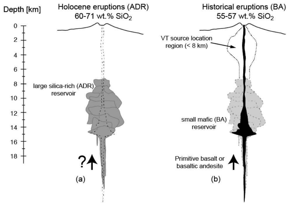
Figure 14. Reconstruction of the magmatic plumbing system beneath Ubinas volcano for (a) the ADR group (post glacial and Holocene), and (b) the BA group (Historical and recent eruptions). The volcano-tectonic (VT) seismic source location comes from Machacca-Puma et al. (2019).
