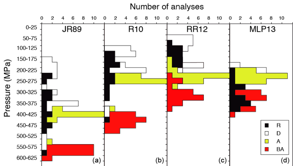
Figure 11. Histograms of amphibole crystallization pressure estimates for Ubina samples (BA: basic andesites;
