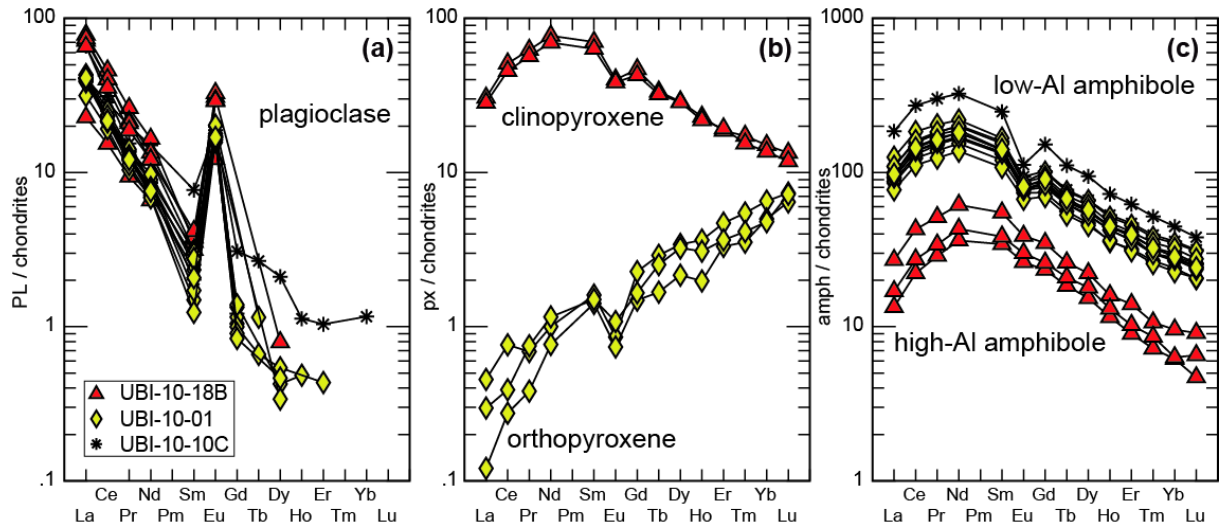
Figure 9. Rare earth element (REE) diagram for selected (a) plagioclase, (b) ortho and clinopyroxene, and (c) amphibole phenocrysts from Ubinas samples. Note that two populations exist for amphibole. Data normalized to chondrite values (Sun and McDonough, 1989). Data correspond to a basaltic andesite (UBI-10-18B), an andesite (UBI-10-01) and a rhyolite (UBI-10-10C).
