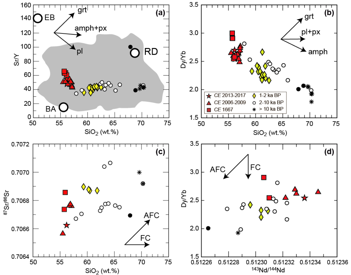
Figure 12. (a, b, c) Sr/Y, Dy/Yb, and ^{87}\text{Sr}/^{86}\text{Sr} vs. silica content. (d) Dy/Yb vs. ^{143}\text{Nd}/^{144}\text{Nd} . The white circles labelled as “BA”, “EB” and “RD” correspond to the three end-members identified by Blum-Oeste and Wörner (2016). BA – calc-alkaline basaltic andesite, EB – shoshonitic enriched basalt, RD – crustal-derived rhyodacite. The grey field corresponds to the CVZ geochemical variation. The arrows in (a, b) show the expected effects of garnet, amphibole and plagioclase-pyroxene fractionation. Note that the only mineral able to efficiently fractionate MREE over HREE (i.e. Dy/Yb) is amphibole. The arrows in (c, d) correspond to theoretical trends for FC and AFC process. Symbols are the same as in Fig. 3.
