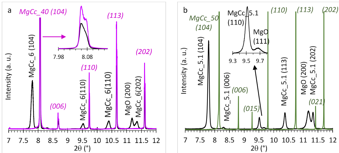
401 Fig. 10 - a) HRXRPD patterns of synthetic MgCc40 recorded at RT (purple line, indexes in italics) and 402 after annealing back to RT (black line). The original material (high-Mg calcite) is partially transformed 403 into low-Mg calcite (~6.0 mol. % MgCO_3 ) and MgO; b) HRXRPD patterns of the synthetic dolomite 404 MgCc50 recorded at RT before thermal processing (green line, and indexes in italics) and at RT after 405 annealing at 1073 K (black line). The original dolomite has been totally transformed into low Mg calcite 406 with ~ 5.1 mol.% MgCO_3 and MgO. [wavelength of \lambda = 0.41068(1) Å (30 keV)] 407 408
