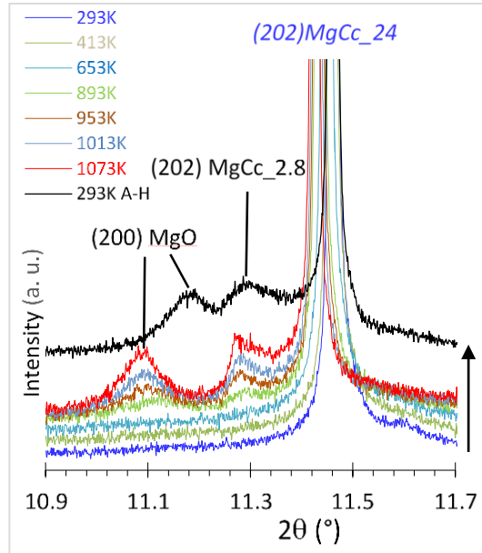
394 Fig. 9 - Selected HRXRPD diffractograms in the 10.9 -11.7 2\theta ( ^{\circ} ) range of the synthetic MgCc24 sample 395 recorded from RT to T=1073 K and then back to RT after heating (293 K A-H), showing (1) the (2 0 2) 396 peaks of untransformed magnesian calcite ( T in the range RT-653 K, indexes in italics) and partially 397 decomposed product (at T > 653 K), and (2) the (2 0 0) peak of MgO resulting from partial decomposition 398 (above 653 K). The black diffractogram collected at RT after annealing is shifted in intensity for clarity 399 (black vertical arrow). [wavelength of \lambda = 0.41068(1) Å (30 keV)] 400
