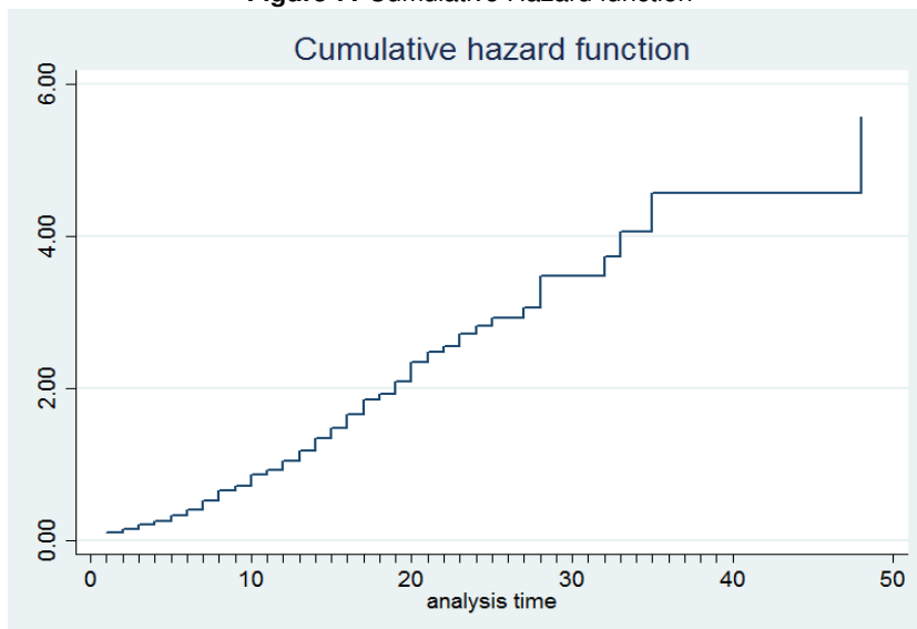
Figure 7: Cumulative Hazard function
