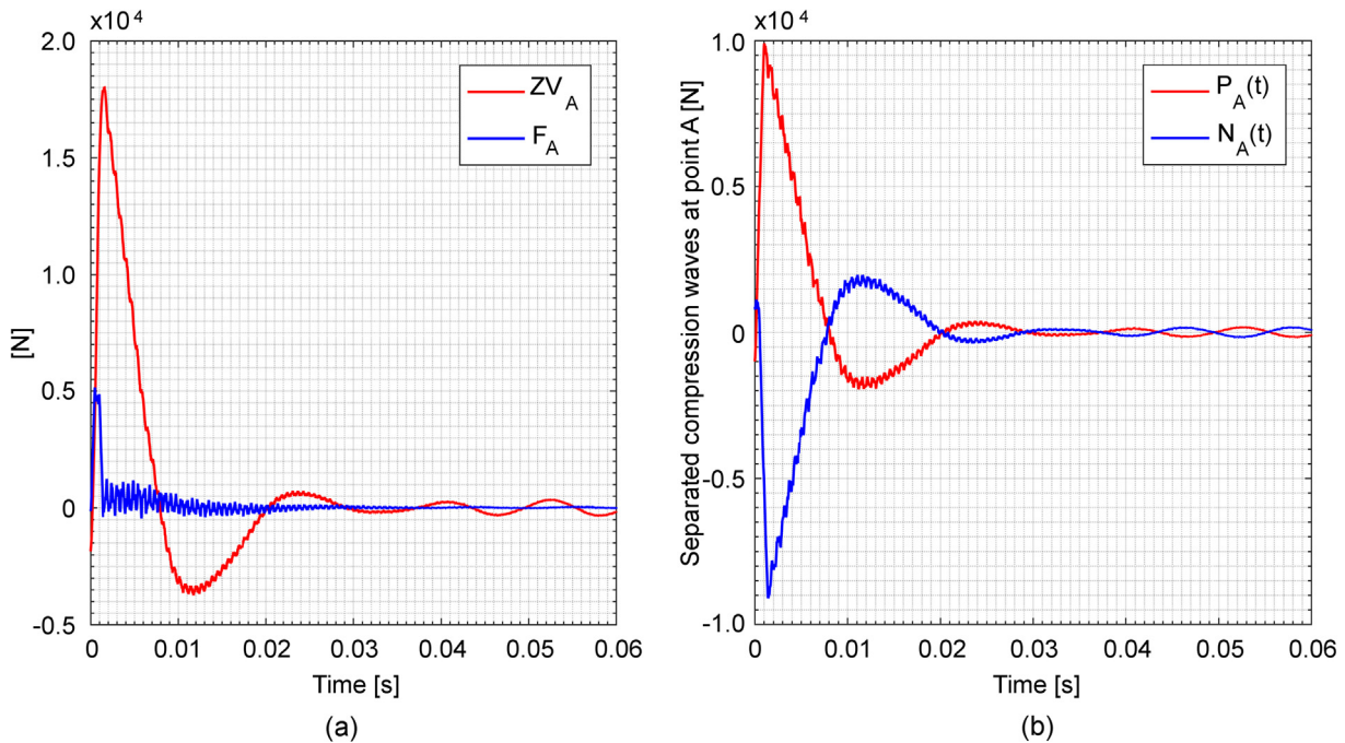
Fig. 6. (a) Measurements at point A, force F_A , and velocity V_A , as functions of time after the impact, and (b) Results of the calculation of elementary compression waves passing point A, as functions of time, after the impact: P_A is the descending wave and N_A is the ascending wave.
