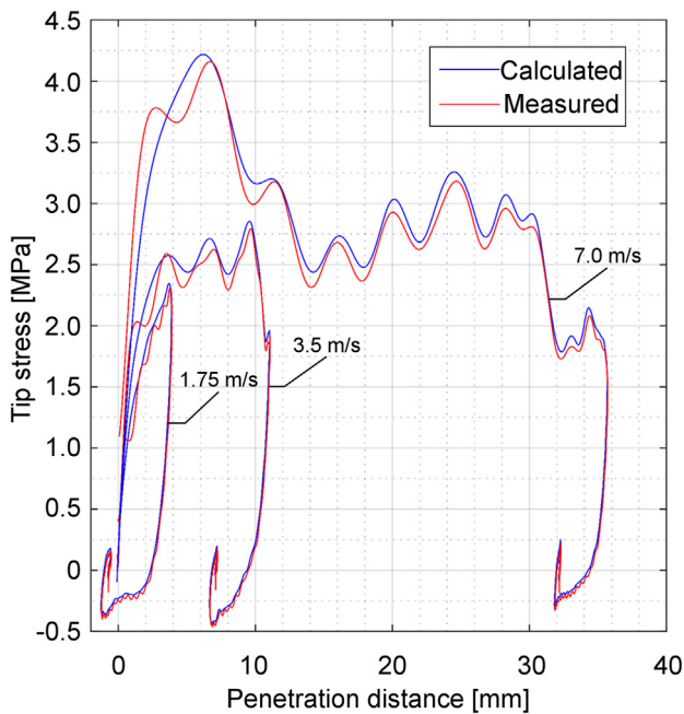
Fig. 7. Comparison of the stress between the tip and the soil for impact velocities of 1.75, 3.5, and 7.0 \text{m s}^{-1} , obtained by the wave separation method (blue line) and actually observed at the tip of penetrometer (red line).
