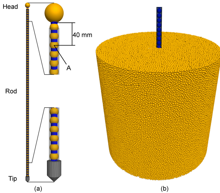
Fig. 4. Numerical model: (a) view of the model representing the penetration test device, based on the Panda 3 specifications, and (b) view of the penetrometer driven in a sample of spheres.
