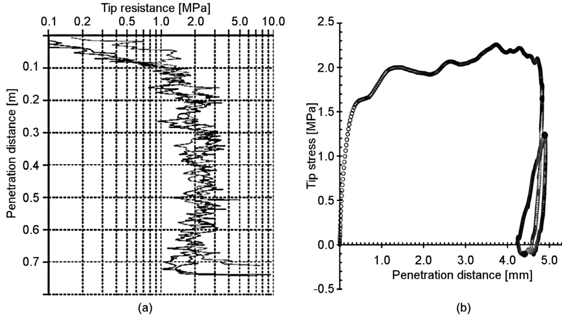
Fig. 1. Results obtained from dynamic penetration Panda 3® tests: (a) for complete tests in terms of tip resistance as a function of depth and (b) for a single impact on the penetrometer in terms of stress on the tip as a function of the tip penetration distance (Benz-Navarrete, 2009).
