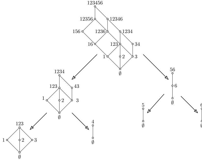
Fig. 7: The H-decomposition of the closure system corresponding to the dihypergraph in Figure 6
