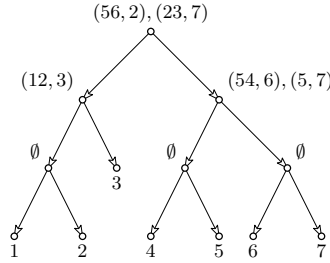
Fig. 3: A H-decomposition for the dihypergraph in Figure 1
