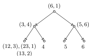
Fig. 6: H-decomposition into H-factors
