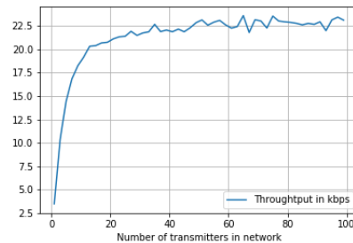
Fig. 5. Average application throughput at the 802.15.4 sink node depending on the number of nodes in network (1 run).
