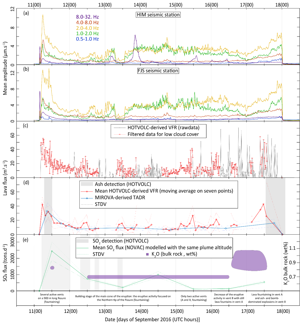
Fig. 2 – (a) and (b) Evolution of the volcanic tremor measured by the HIM and FJS seismic stations respectively. (c) And (d) represent the evolution of the lava fluxes by the HOTVOLC system (raw data, filtered data, average) and the MIROVA system. Periods with ash detected by HOTVOLC are displayed in grey areas. (e) Evolution of the SO 2 flux measured by the NOVAC stations. Periods with SO 2 detected by HOTVOLC are displayed in grey areas.
