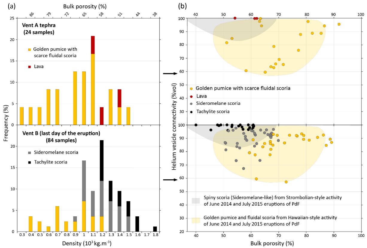
Fig. 6 – (a) Density and porosity measurements, displayed in histograms and normalized to the total number of samples for vent A and vent B. (b) Helium vesicle connectivity measurements vs. porosity.
