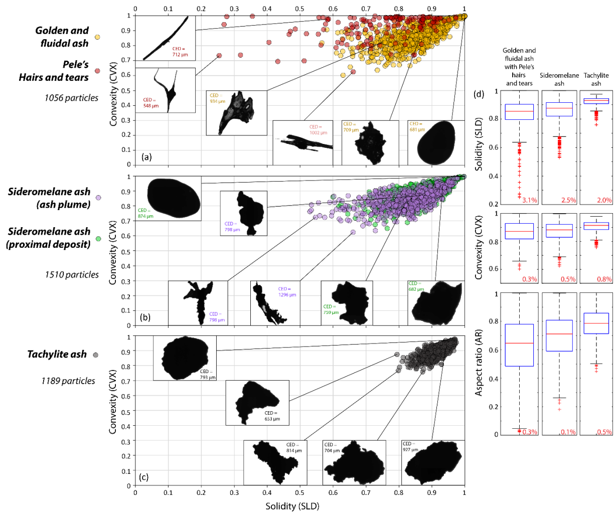
Fig. 8 – Morphometric (APASH, solidity vs. convexity) dataset of each ash component at 0.5-1 \phi grain size fraction. (a) Golden/fluidal ash with Pele's hairs and tears, (b) sideromelane ash and (c) tachylite ash. (d) Statistical analysis of each component dataset on boxplots for solidity, convexity and aspect ratio of the particles. Middle red lines represent the median, blue boxes represent all the particles between the 25 th and 75 th percentiles (englobes 50% of the dataset), boxplot whisker boundaries represent 2.7 \sigma of the data, and red crosses represent each ash particles outside this boundary (outliers).
