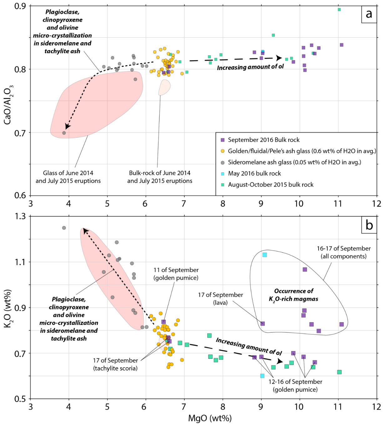
Fig. 9 – Bulk rock and in-situ glass compositions (MgO vs. CaO/Al 2 O 3 ) of the eruptive products.
