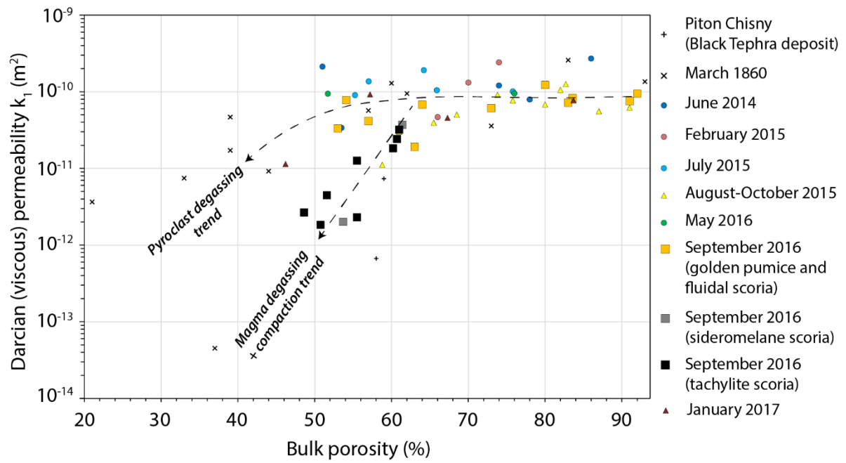
Fig. 7 – Darcian permeability ( k_1 ) vs. porosity of several samples from different eruptions of PdF.
