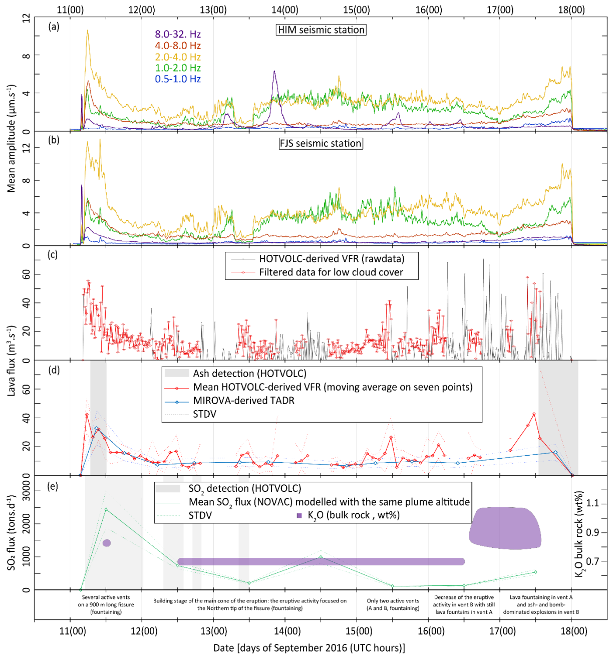
Fig. 2 – (a) and (b) Evolution of the volcanic tremor measured by the HIM and FJS seismic stations respectively. (c) And (d) represent the evolution of the lava fluxes by the HOTVOLC system (raw data, filtered data, average) and the MIROVA system. Periods with ash detected by HOTVOLC are displayed in grey areas. (e) Evolution of the SO 2 flux measured by the NOVAC stations. Periods with SO 2 detected by HOTVOLC are displayed in grey areas.
