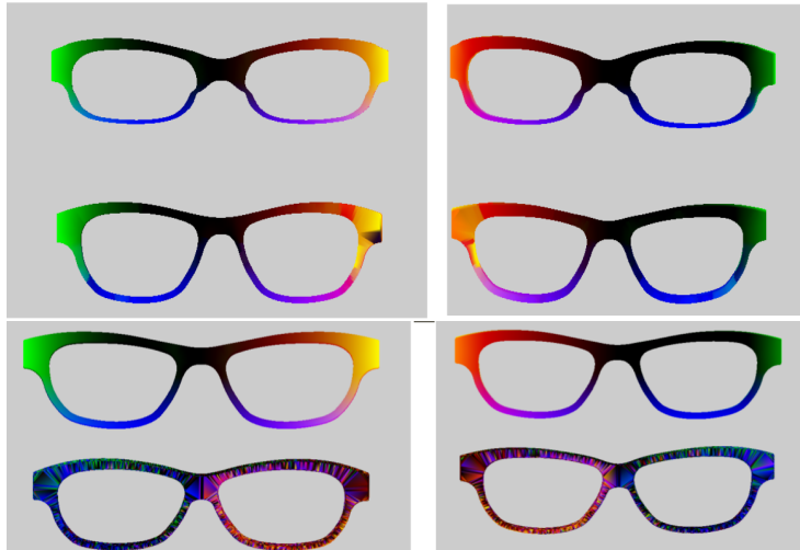
Figure 4: Functional Maps used on our glasses. First column shows front of glasses and second columns the back. Firsrt rows is between glasses b) and a). Second rows is between glasses a) and c). Same colors should indicate correspondant regions.
