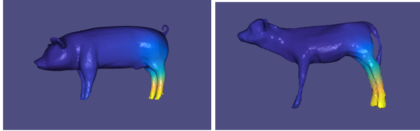
Figure 7: eigenfunction of Laplace-Beltrami that highlights the back legs of the two animals. For the pig, it is the 4th eigenfunction whereas for the veal it is the 3rd.
