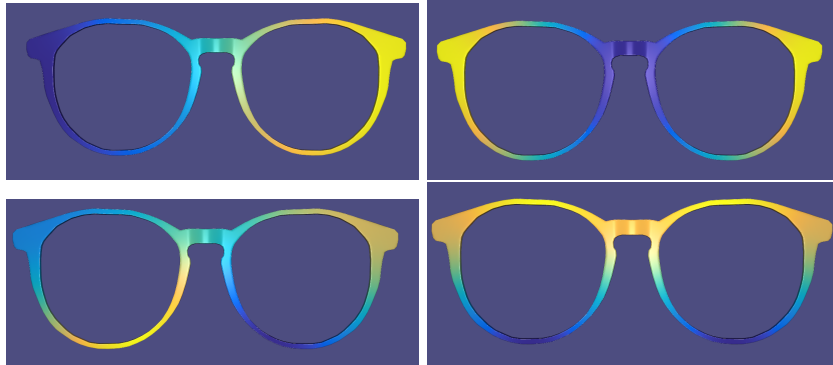
Figure 5: On first row : 1st, 2nd eigenfunctions of Laplace-Beltrami. On second row : 3rd and 4th eigenfunctions of Laplace-Beltrami.
