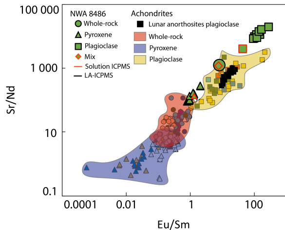
Figure 2: Eu/Sm versus Sr/Nd plot. Plagioclase, pyroxene and whole-rock data for achondrites are represented along with NWA 8486 (green) and lunar anorthosites plagioclase (black) for comparison. Fields show the range of pyroxene (blue), plagioclase (yellow) and whole-rock (red) compositions. Data are from too many sources to cite here.
