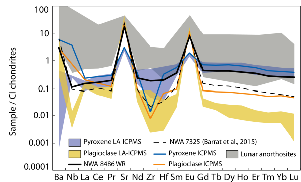
Figure 1: In-situ and solution trace element composition of minerals and whole-rock (WR) of NWA 8486 normalised to CI chondrites [8]. Lunar anorthosites range is plotted for comparison (data from [9, 10, 11]).
