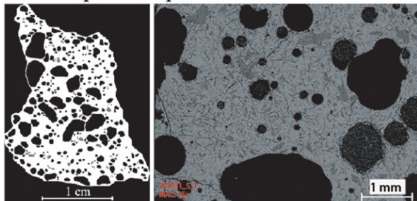
Figure 4. Binary images of thin sections and backscattered electron images for (A) near-vent sample of day 1, plus (B) shear zone, and (C) plug zone of sample taken on day 2 of the July–August 2015 eruption of Piton de la Fournaise (La Réunion, France) (white—matrix, gray—phenocrysts, and black—vesicles).
