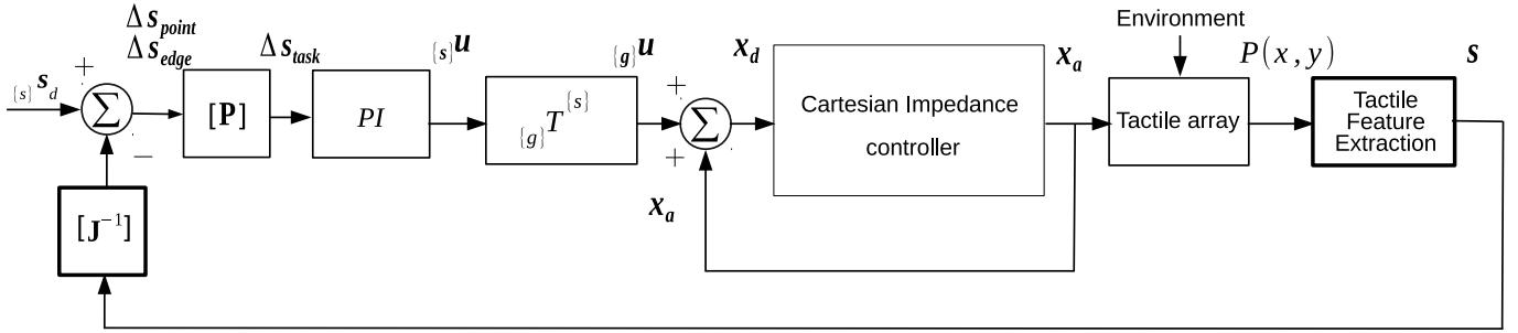
Figure 8: Block diagram of the external hybrid tactile-position controller. The Cartesian impedance controller is a part of a robot with its default stiffness and damping parameters.
