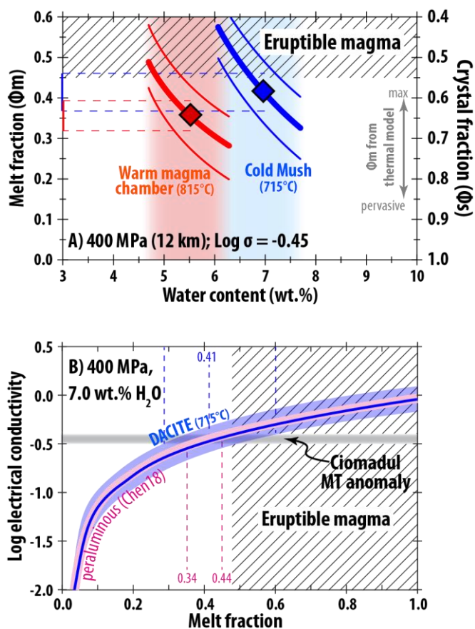
536 Figure 9: Melt fraction beneath Ciomadul volcano. (A) The melt fraction and water content respecting the electrical 537 anomaly (Log electrical conductivity -0.45) observed by magnetotelluric survey (Harangi et al., 2015b) for both reservoir 538 and mush cases. The curves are truncated according to the possible range of water content constrained by the petrology
