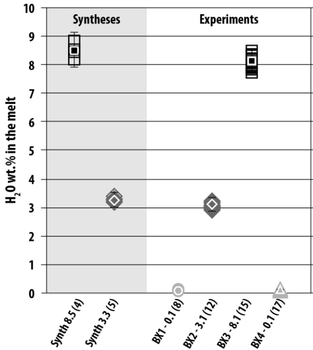
Figure 2: Water content of dacitic glasses after hydration (Syntheses) and of experimental glasses after electrical conductivity measurements ("Experiments"). Empty symbols correspond to single analyses and full symbols to the average. The water variation before and after in situ electrical conductivity experiments is neglectable (lower than 5%).
