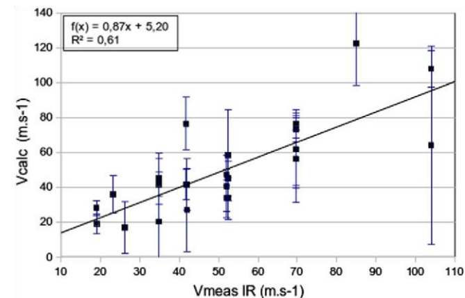
Fig. 11. Velocity calculated from the rectangular FOV synthetic signal ( V_{\text{calc}} ), compared to values measured on thermal videos ( V_{\text{meas IR}} ). Results are in good agreement, although the error can be very important.
