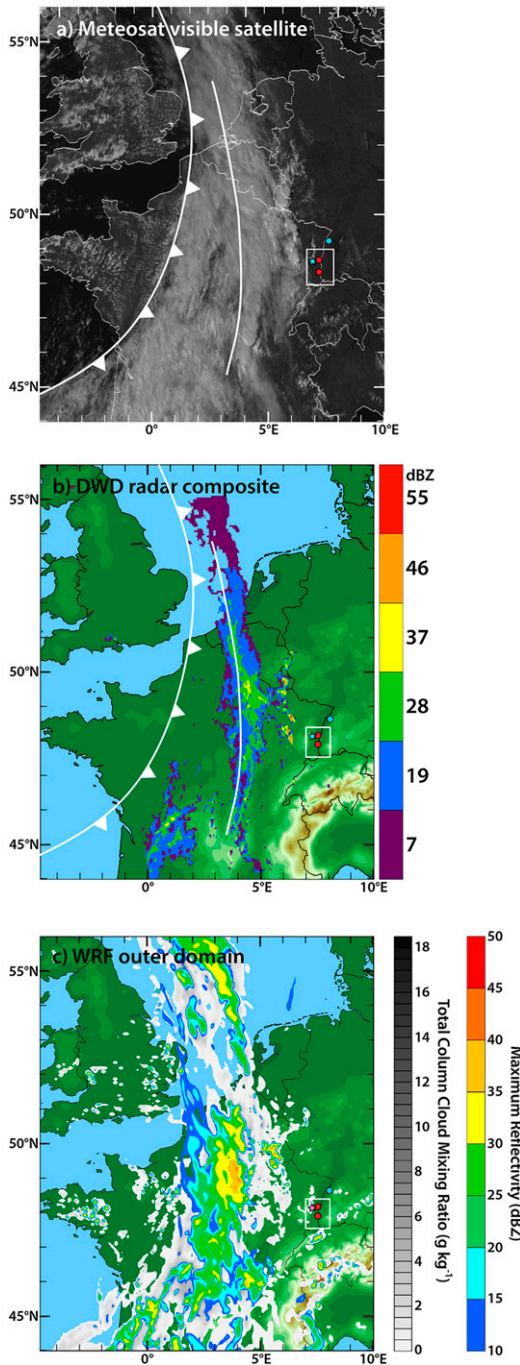
FIG. 5. Comparison of 1400 UTC 6 Aug 2007 (a) Meteosat visible satellite image, (b) DWD radar composite, and (c) WRF outer domain simulation. The cold front and trough locations in (a),(b) are approximated. White dual-Doppler box to be shown in Fig. 11 is shown in all panels as are red dots showing locations of DOW2 and DOW3. The Achern Supersite location is the blue dot in the northeastern Rhine Valley. Blue star is the CI location observed in (a),(b) and pink star is the WRF simulated CI location in (c). Colored shading is maximum radar reflectivity (dBZ): observed in (b) and simulated in (c). Gray shading in (c) is total column-integrated cloud water mixing ratios ( \text{g kg}^{-1} ).
