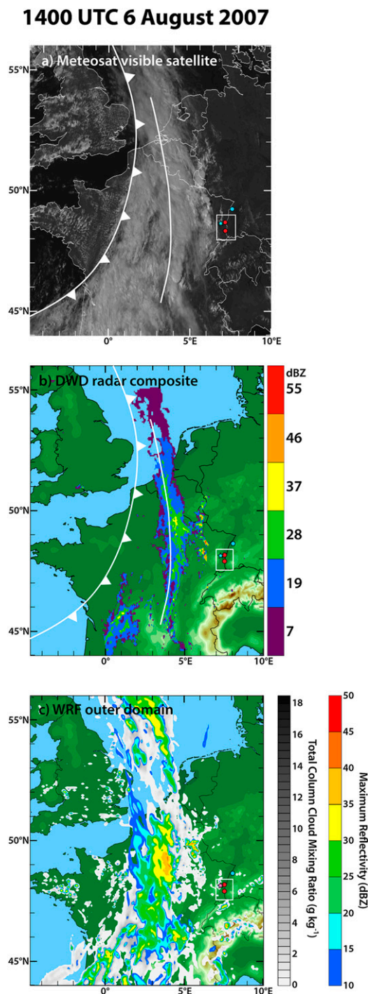
FIG. 5. Comparison of 1400 UTC 6 Aug 2007 (a) Meteosat visible satellite image, (b) DWD radar composite, and (c) WRF outer domain simulation. The cold front and trough locations in (a), (b) are approximated. White dual-Doppler box to be shown in Fig. 11 is shown in all panels as are red dots showing locations of DOW2 and DOW3. The Achern Supersite location is the blue dot in the northeastern Rhine Valley. Blue star is the CI location observed in (a), (b) and pink star is the WRF simulated CI location in (c). Colored shading is maximum radar reflectivity (dBZ): observed in (b) and simulated in (c). Gray shading in (c) is total column-integrated cloud water mixing ratios ( \text{g kg}^{-1} ).
