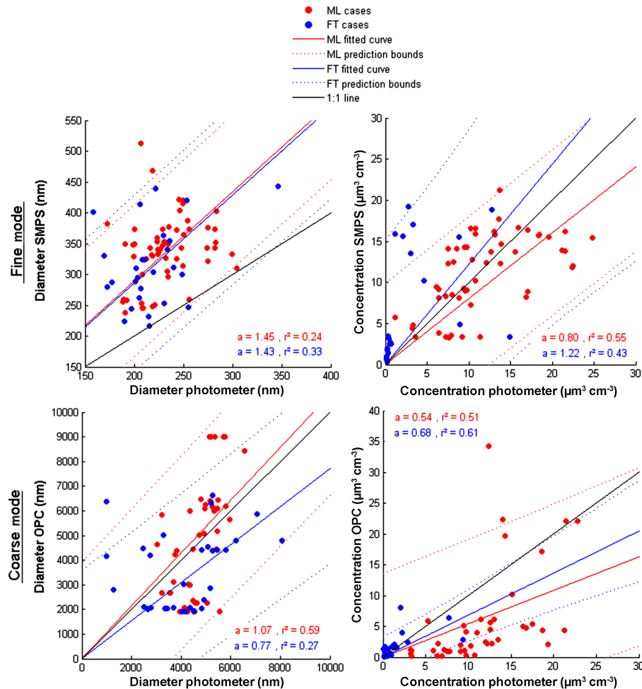
Figure 7. Scatter plot of fine and coarse mode modal diameters, and volume concentrations after applying the ML and FT contribution factors to sun photometer concentrations. Blue fit and markers are for FT data and red fit and markers for ML data.
