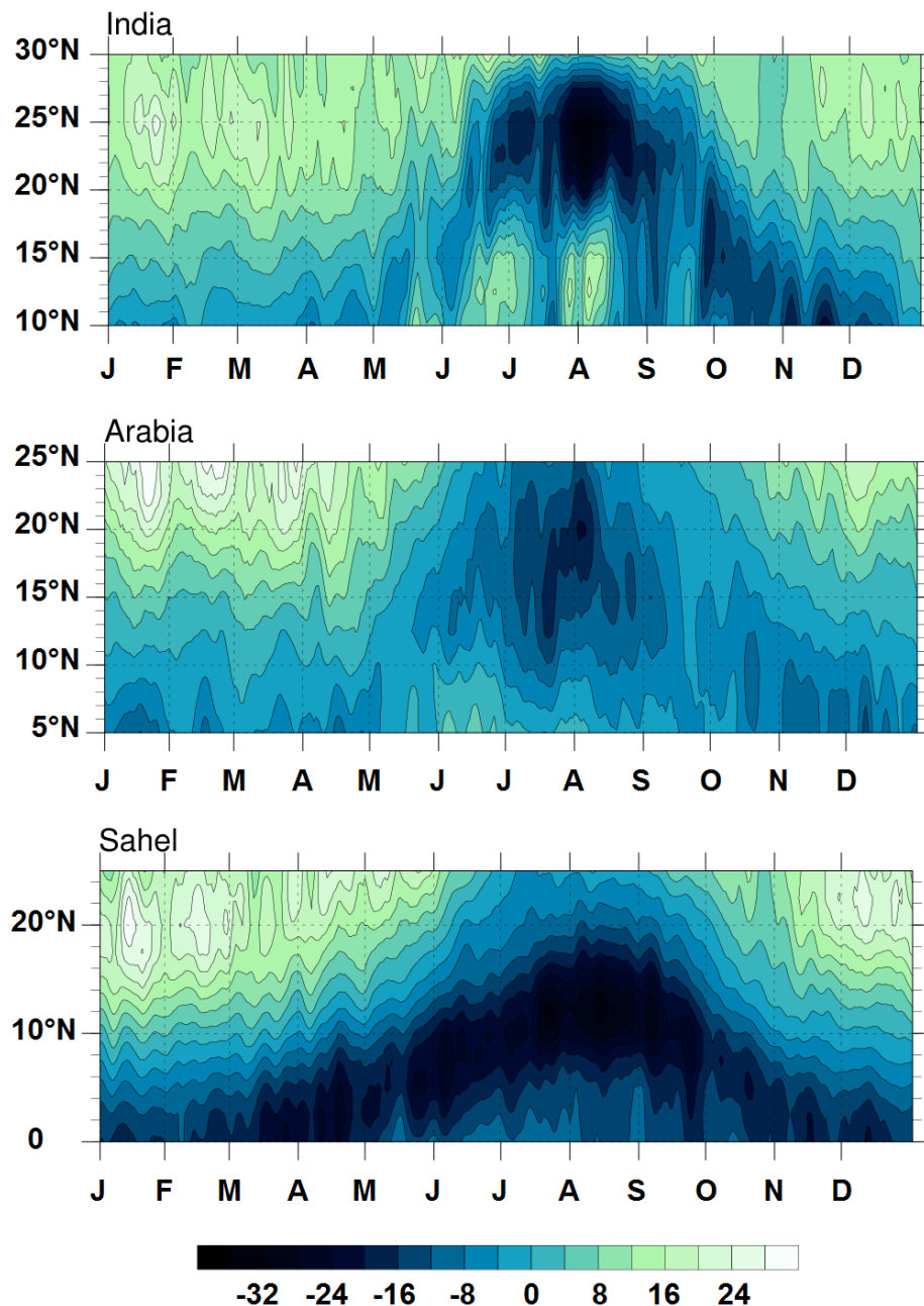
Figure 8. Time-latitude plots of zonal fluxes (in \text{kg}\cdot(\text{m}\cdot\text{s})^{-1} ) between January to December averaged over the period 1998–2008 above India ( 70\text{--}90^\circ\text{ E} , top), Arabia ( 45\text{--}60^\circ\text{ E} middle), and Sahel ( 10^\circ\text{ W}\text{--}20^\circ\text{ E} , bottom). Data have been filtered using a 5 day moving average.
