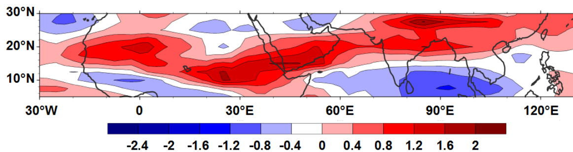
Figure 3. Climatology of the wind divergence (in day^{-1} ) from 500 to 300 hPa resulting from ECMWF ERA-Interim averaged from June to September over the period 1998–2008 between 0\text{--}30^\circ N and 30^\circ W– 130^\circ E.
