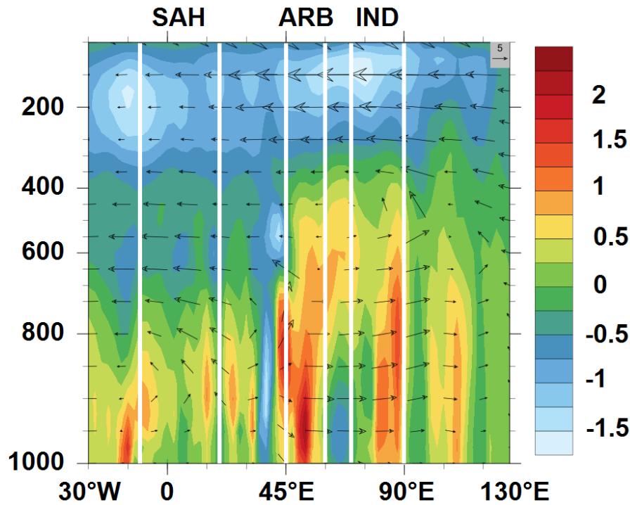
Figure 2. Zonal cross section of the zonal and vertical component of the wind (vectors) and the relative vorticity ( \times 10^5, s^{-1} colors) averaged between 10\text{--}23^\circ N from June to September over the period 1998–2008, and from 30^\circ W to 130^\circ E. The longitudes of SAH, ARB, and IND regions are marked by white vertical lines.
