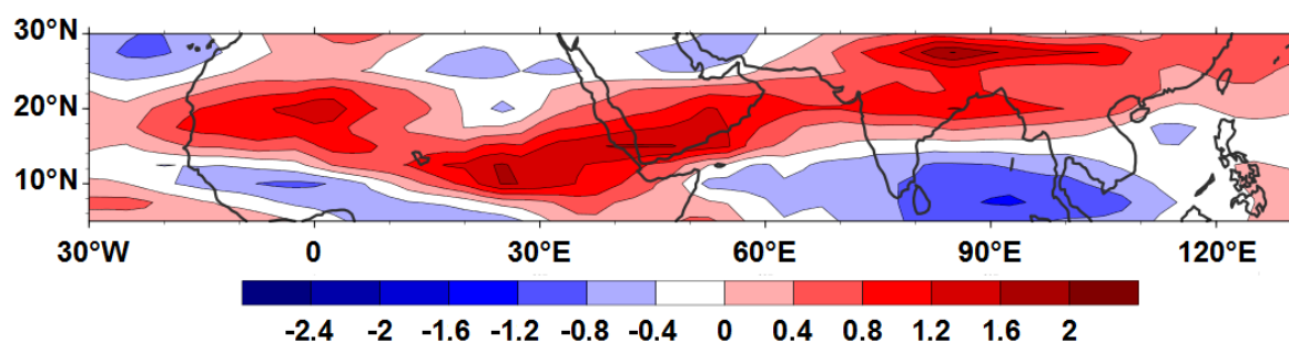
Figure 3. Climatology of the wind divergence (in day^{-1} ) from 500 to 300 hPa resulting from ECMWF ERA-Interim averaged from June to September over the period 1998–2008 between 0^{\circ} – 30^{\circ} N and 30^{\circ} W– 130^{\circ} E.
