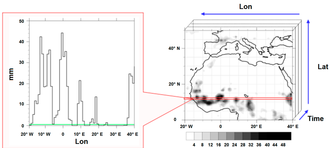
Figure 2. (Right) Lat × Lon + Time map of precipitation in mm/day between 0–50° N and 20° W–40° E over 4018 days (1998–2008) obtained from daily GPCP rainfall data. (Left) transect at 12° N showing rainfall as function of longitude during one day. The threshold equal to 0.1 mm is marked by a green line.
