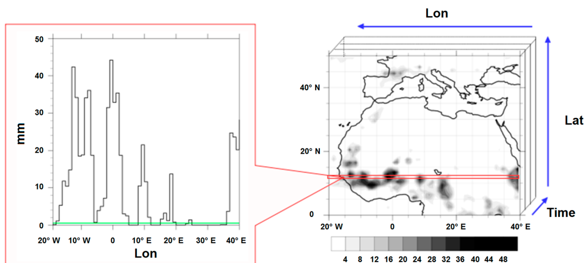
Figure 2. (Right) Lat \times Lon + Time map of precipitation in mm/day between 0^{\circ} – 50^{\circ} N and 20^{\circ} W– 40^{\circ} E over 4018 days (1998–2008) obtained from daily GPCP rainfall data. (Left) transect at 12^{\circ} N showing rainfall as function of longitude during one day. The threshold equal to 0.1 mm is marked by a green line.
