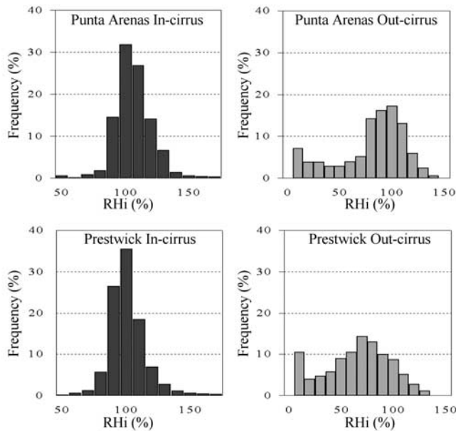
Figure 3. Histograms of RH_i measurement from Punta-Arenas and Prestwick, inside and outside cirrus clouds. Inside clouds there are 51% of the data with RH_i > 105\% at Punta Arenas compared to 31% at Prestwick. For each location, the frequency is with respect to total number of data, inside and outside cirrus respectively.
