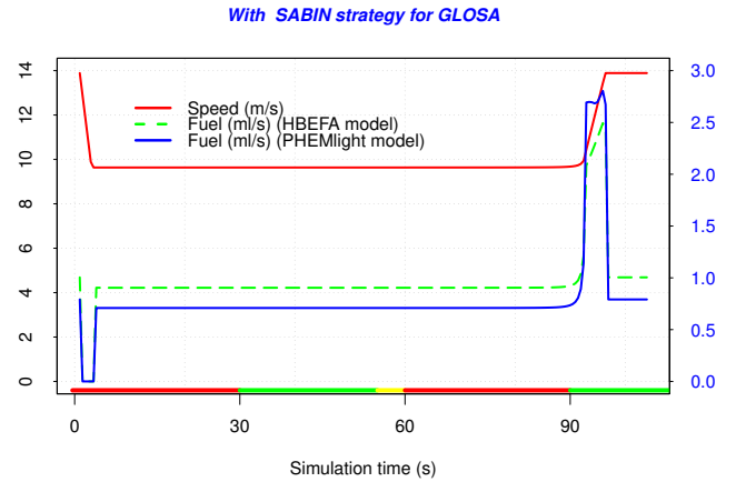
Fig. 5. Fuel consumption and speed comparison.
