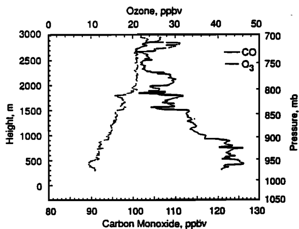
Figure 6. O 3 (dashed line) and CO (solid line) species mixing ratio profiles obtained during the sounding of Figure 4 [from Ritter et al. , 1990].
