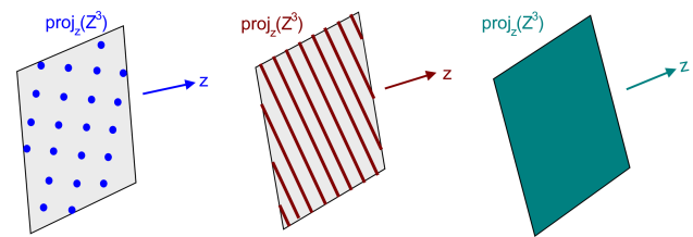
Fig. 17 On the left, the projection of \mathbb{Z}^3 in the z direction if the rational dimension of E_z = \{q \cdot z | q \in \mathbb{Q}^d\} is 1. It means that the z direction is rational and the projection of the lattice is a lattice of dimension 2. In the middle, the rational dimension of E_z = \{q \cdot z | q \in \mathbb{Q}^d\} is 2. We have a rational linear relation between the coordinates of z . The projection of the lattice \mathbb{Z}^3 in the z direction is dense on equidistant parallel lines. On the right, if \dim_{\mathbb{Q}}(E_z) = 3 , there exists no rational linear relation between the coordinates of z . The projection of the lattice \mathbb{Z}^3 is dense in the plane of projection.
