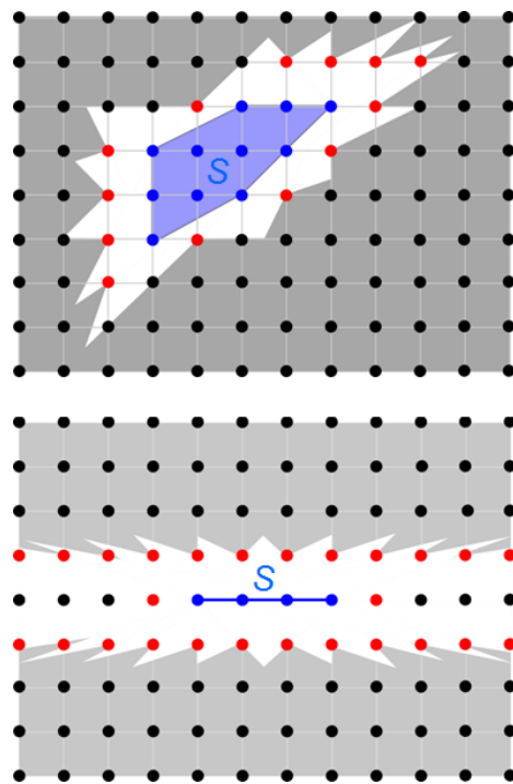
Fig. 10 Two lattice sets S (deep blue), their convex hulls (blue), their crown (white), their lattice jewels (red points) and for each, the shadow (grey) of \mathbb{Z}^2 \setminus S .
