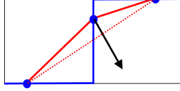
Figure 10: The polygonal curves of minimal length going through a sequence of edges with each time, previous and next edges on both sides of the middle edge, cannot have an angle at a vertex unless it is on the boundary of the edge. Hence the vertices of the curve can only be integer points.
