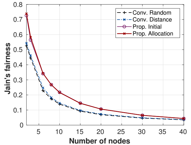
Fig. 4. Jain's fairness metric, proposed and baseline algorithms
