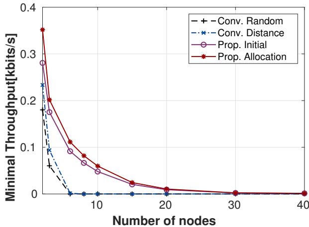
Fig. 2. Minimal short-term average rates, proposed and baseline algorithms
