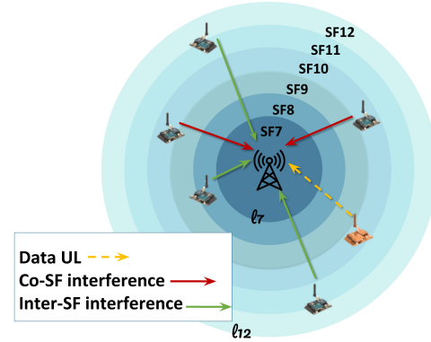
Fig. 1. LoRa system, with end-devices transmitting simultaneously
