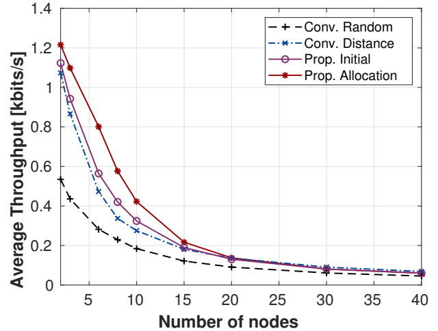
Fig. 3. Average network throughput, proposed and baseline algorithms
