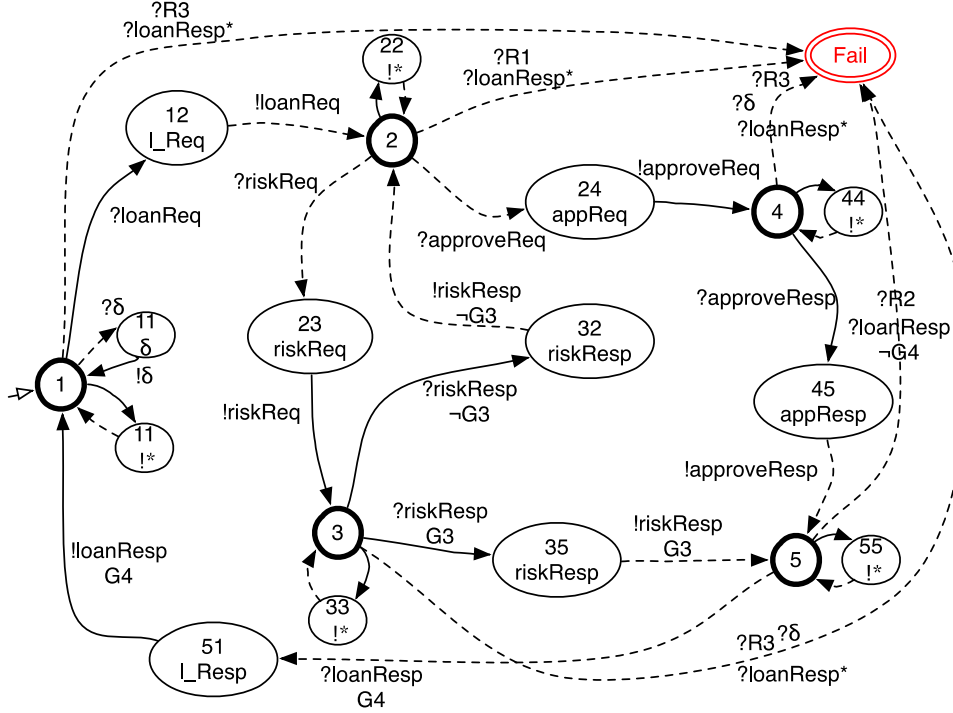
Figure 4: A Proxy-tester.
