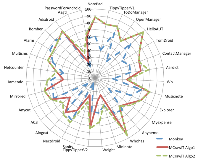
Figure 13: Code coverage comparison (in %)
